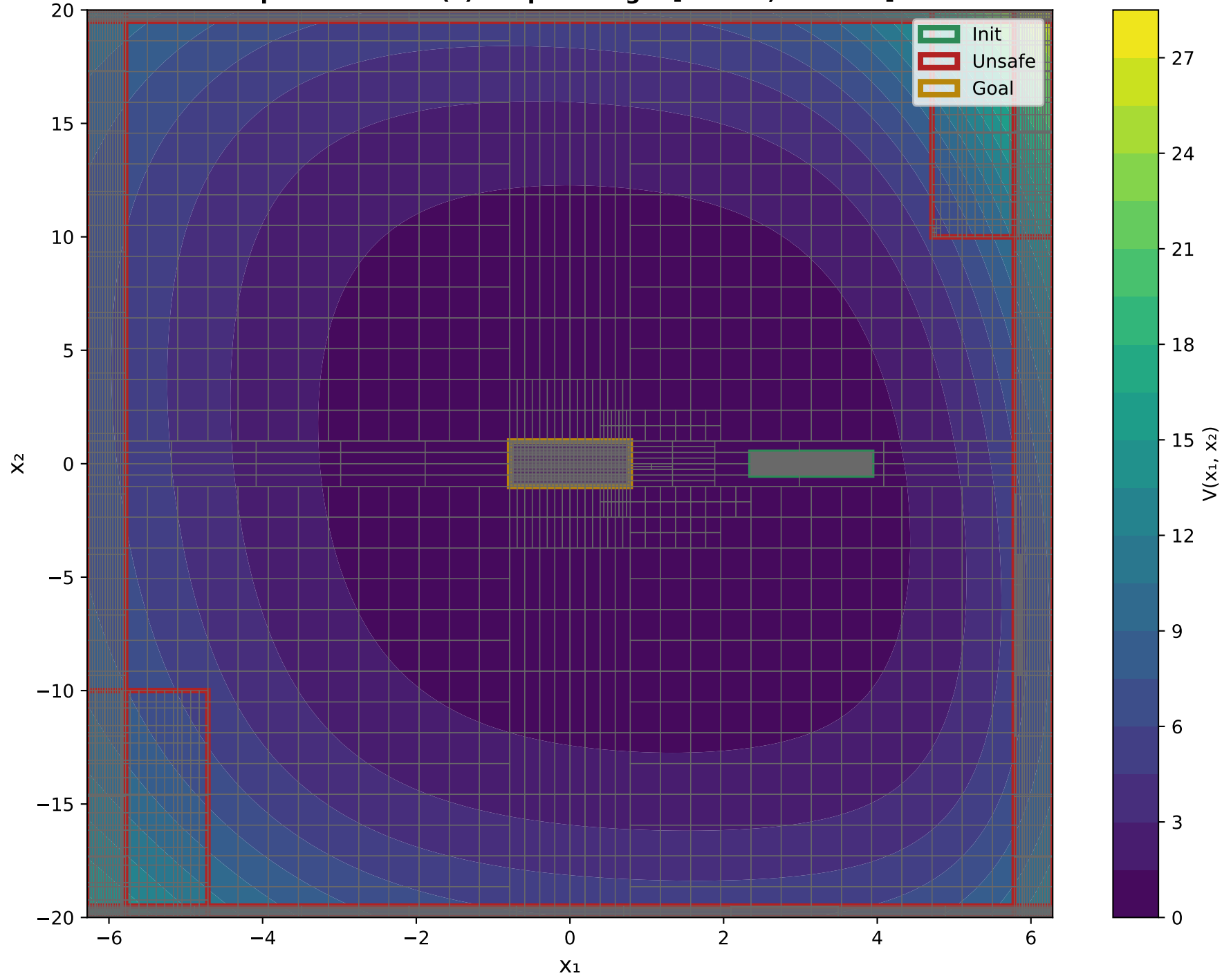
X 1 VS X 2 Epoch: 1000 - V(x) Output Range: [0.0604, 27.5514]
