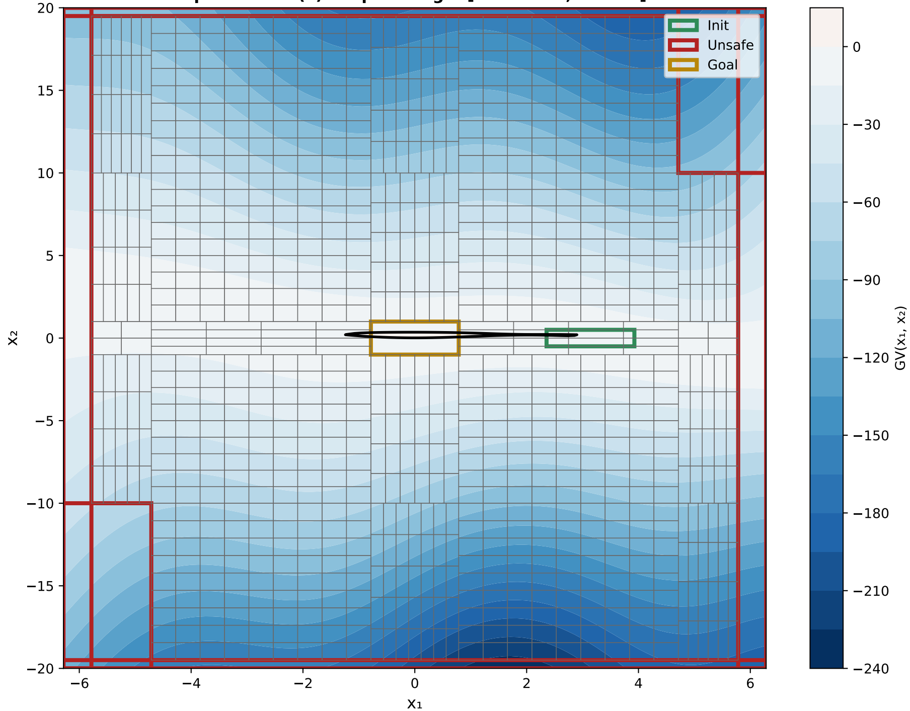
X 1 VS X 2 Epoch 0 - GV(x) Output Range: [-234.2059, 0.5143]
