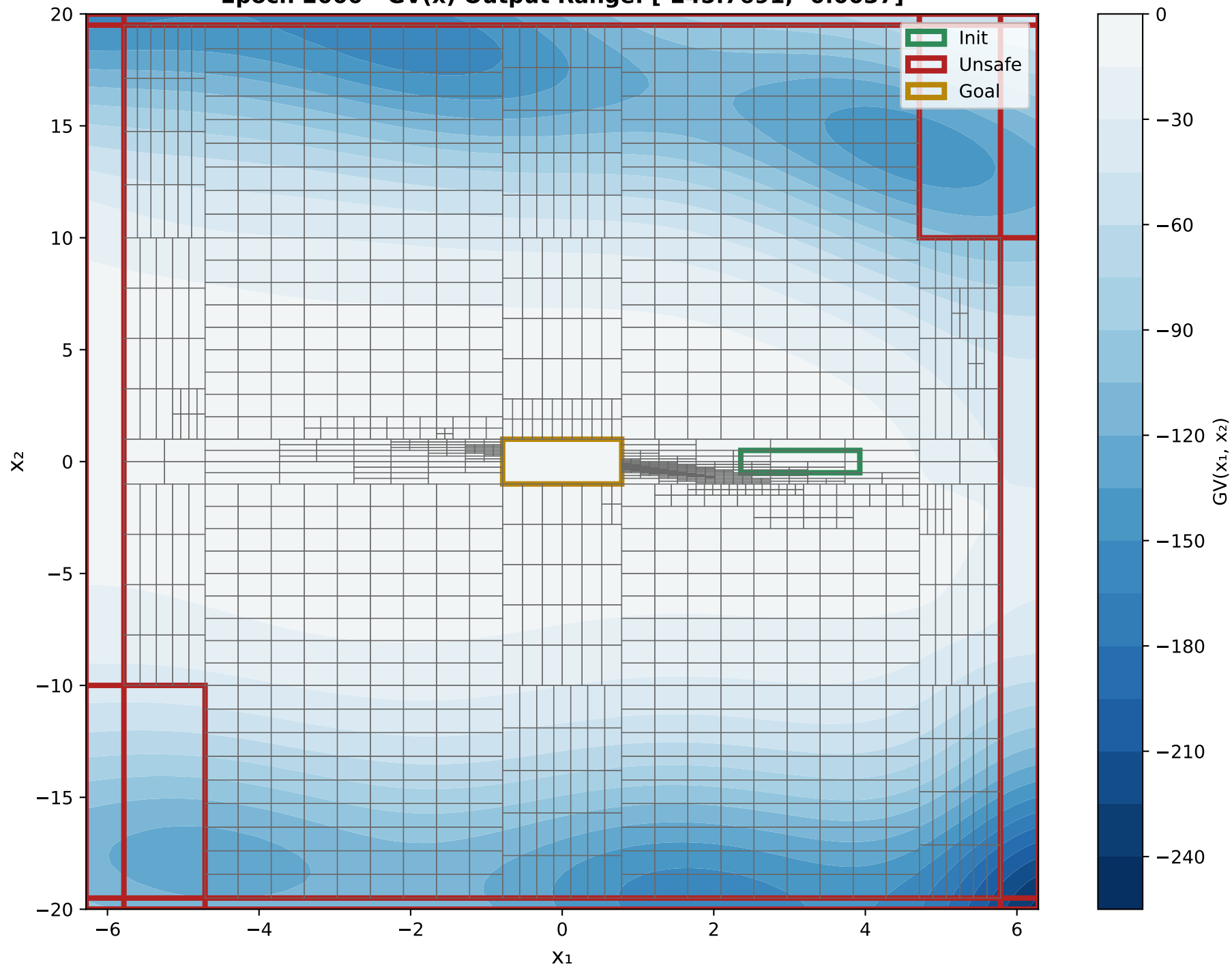
X 1 VS X 2 Epoch 2000 - GV(x) Output Range: [-245.7691, -0.0037]
