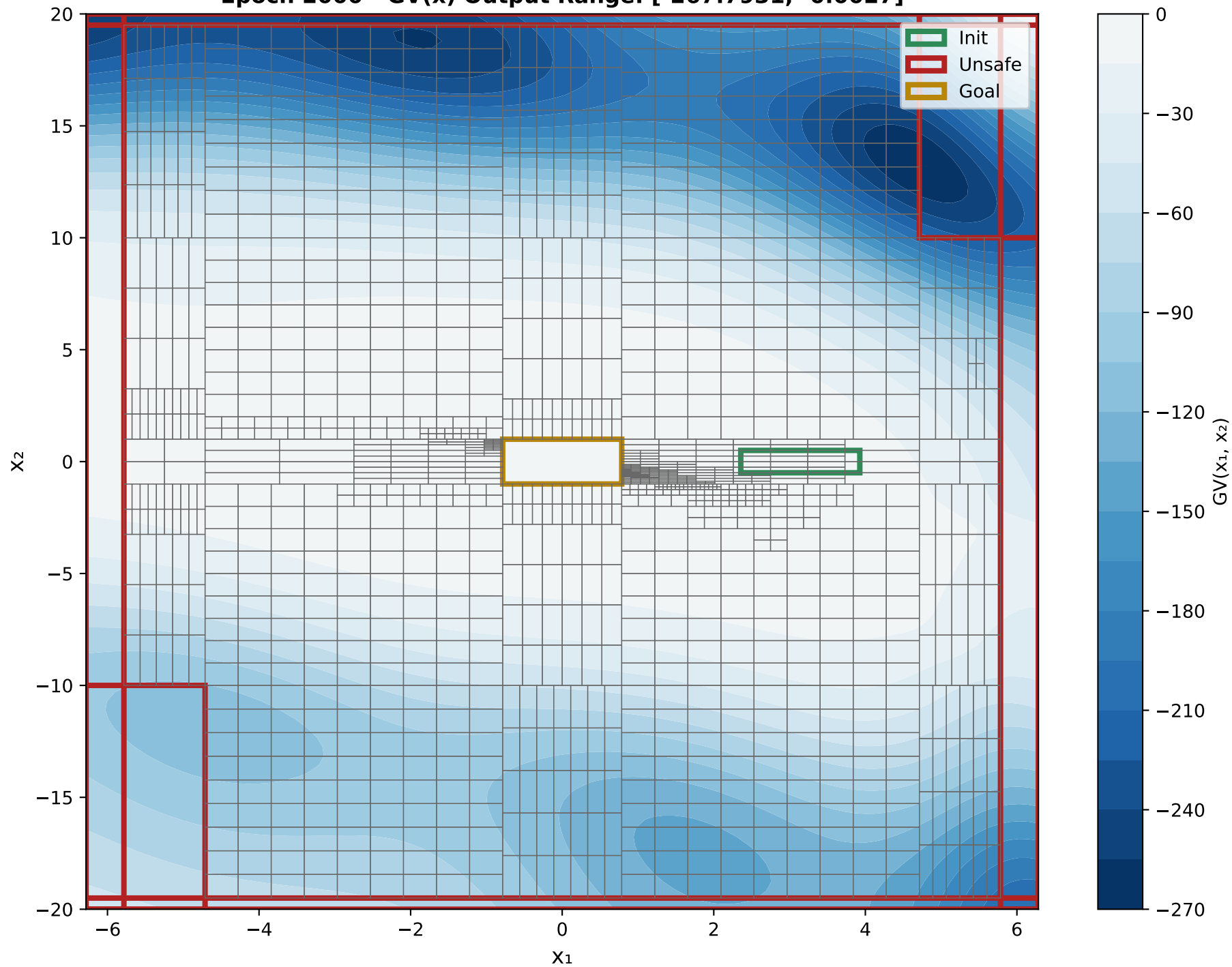
X 1 VS X 2 Epoch 2000 - GV(x) Output Range: [-267.7931, -0.0027]
