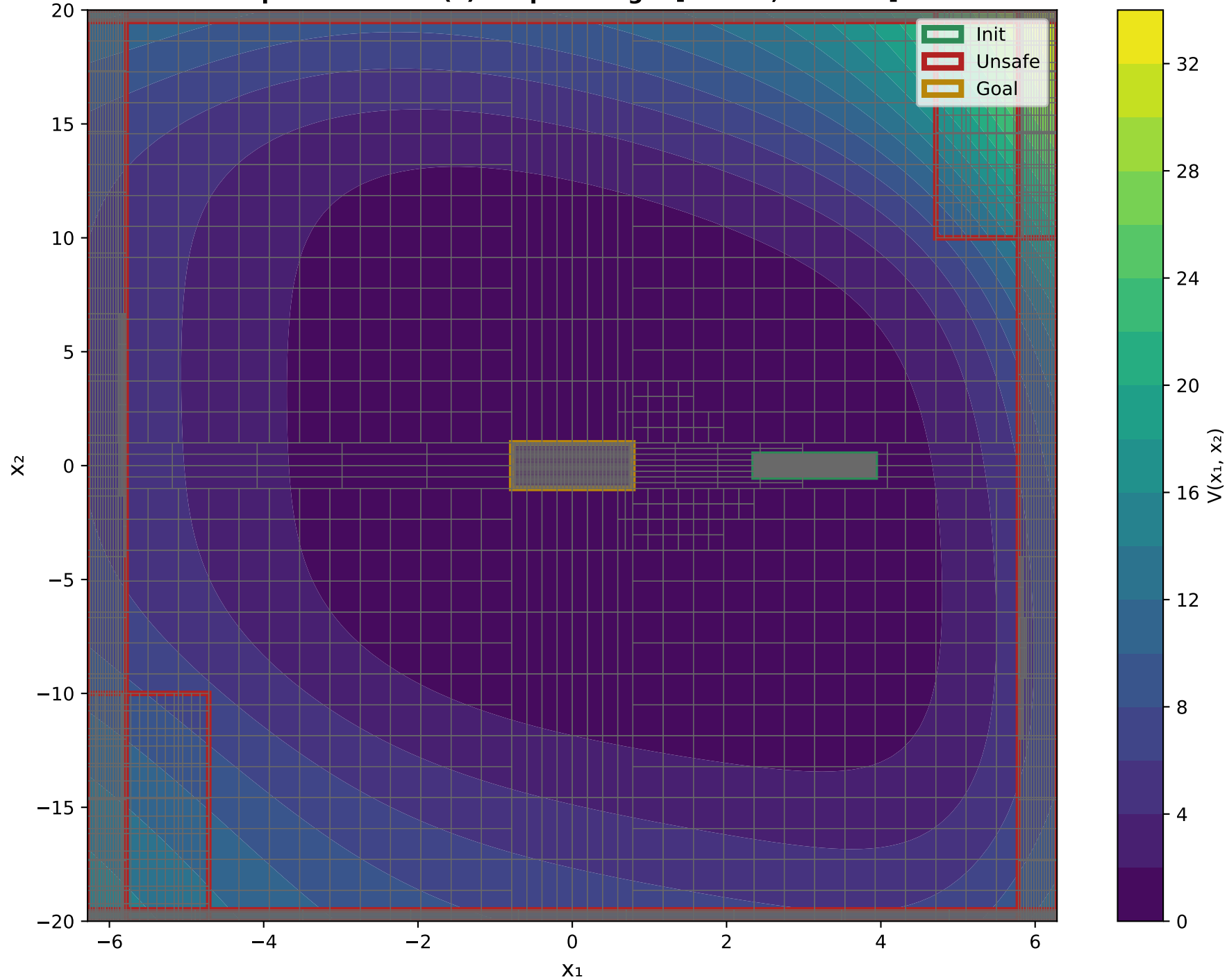
X 1 VS X 2 Epoch: 2000 - V(x) Output Range: [0.0998, 32.3646]
