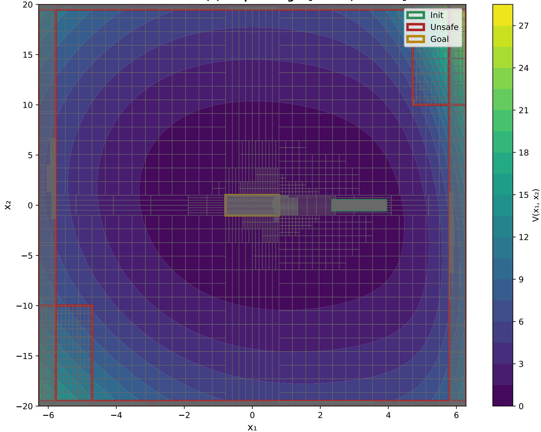
X 1 VS X 2 Final Evaluation - V(x) Output Range: [0.0890, 27.0206]
