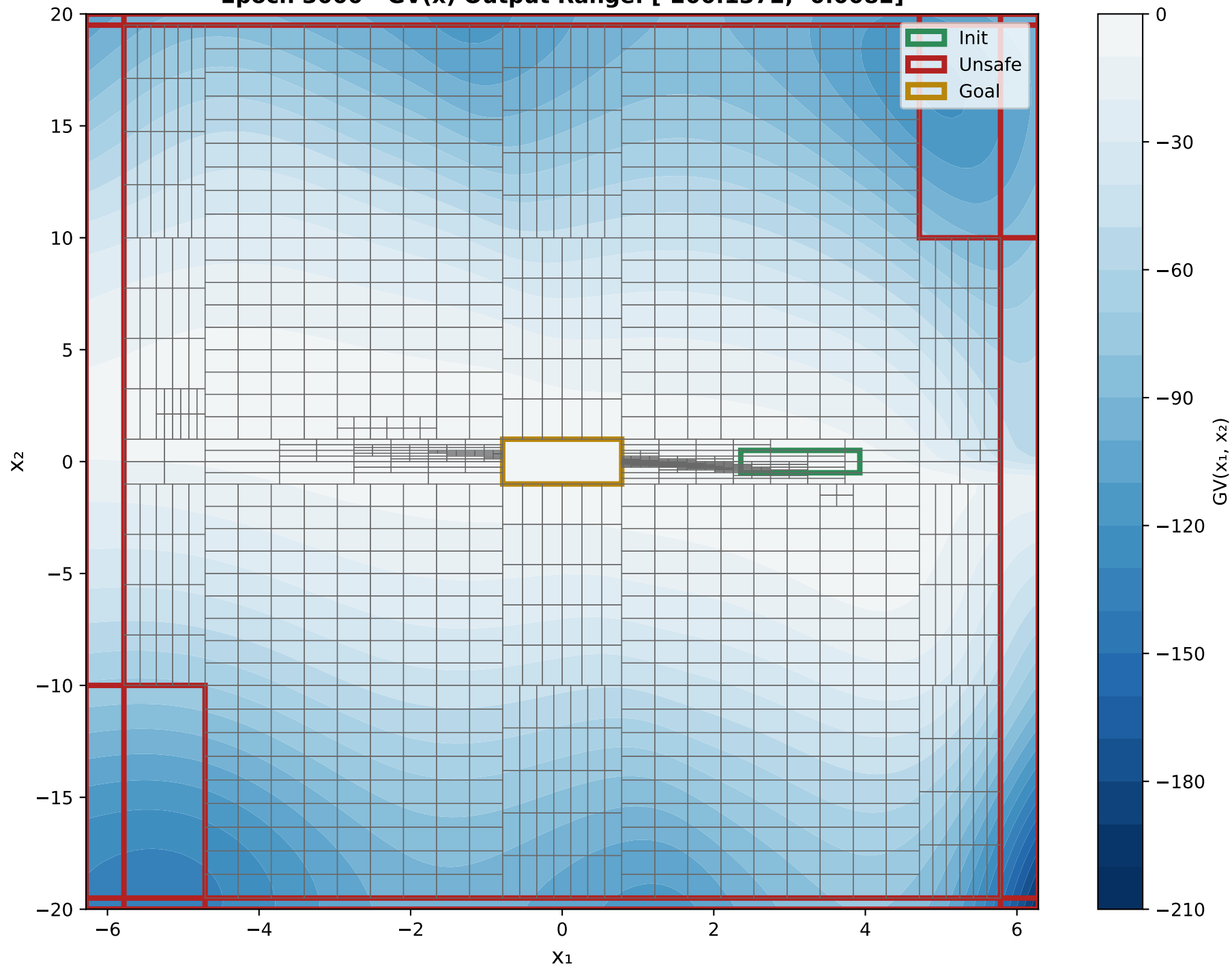
X 1 VS X 2 Epoch 3000 - GV(x) Output Range: [-200.1372, -0.0082]
