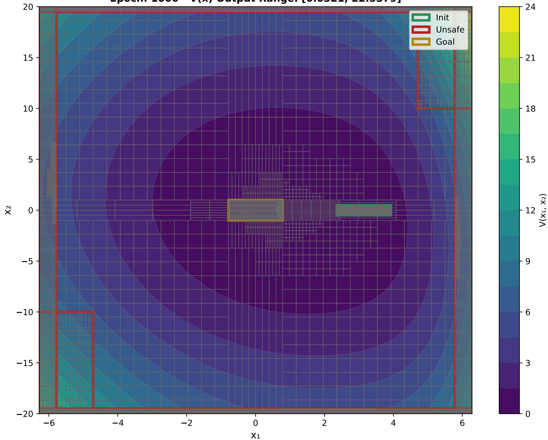
X 1 VS X 2 Epoch: 1000 - V(x) Output Range: [0.0321, 22.5379]
