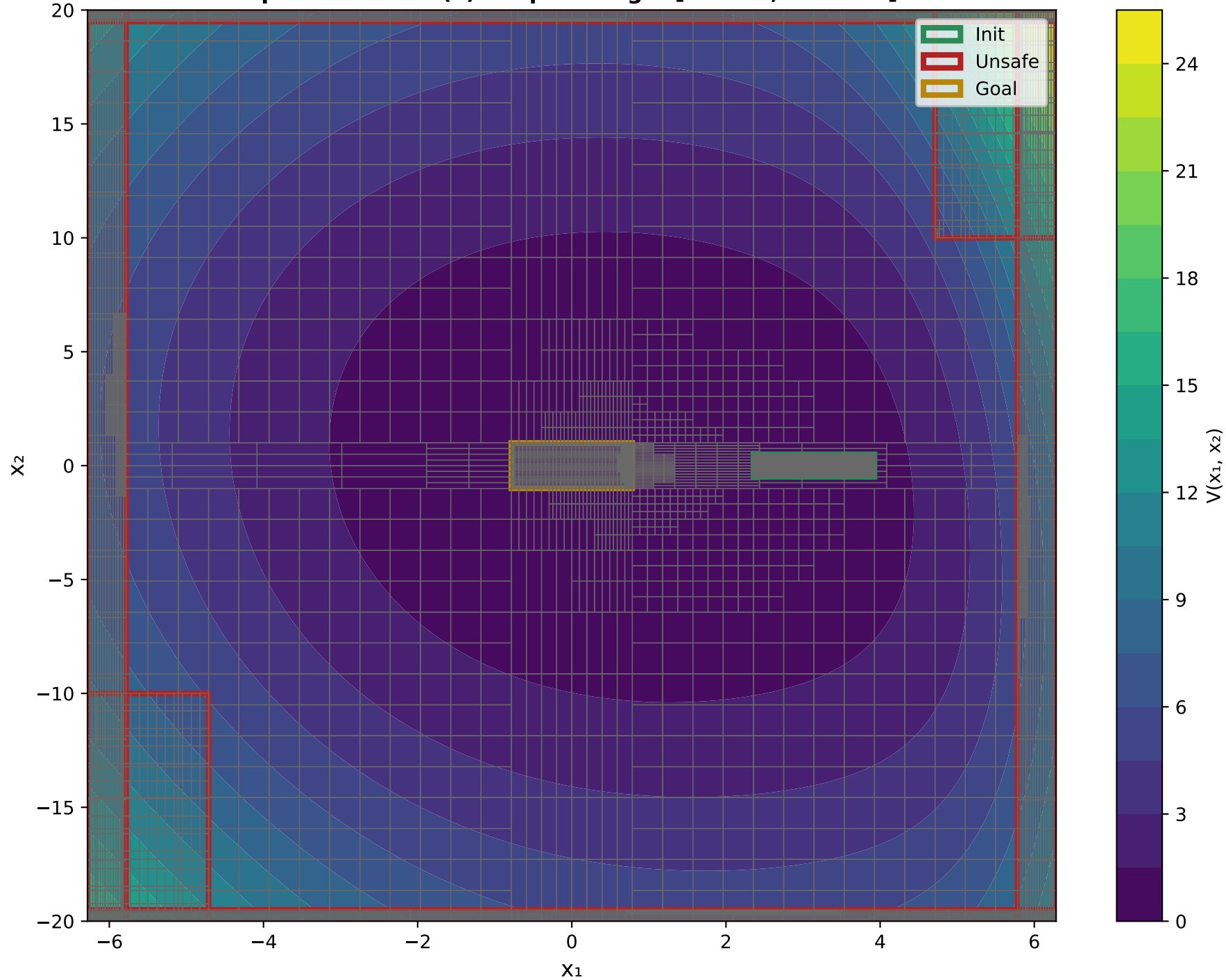
X 1 VS X 2 Epoch: 2000 - V(x) Output Range: [0.0634, 25.1118]
