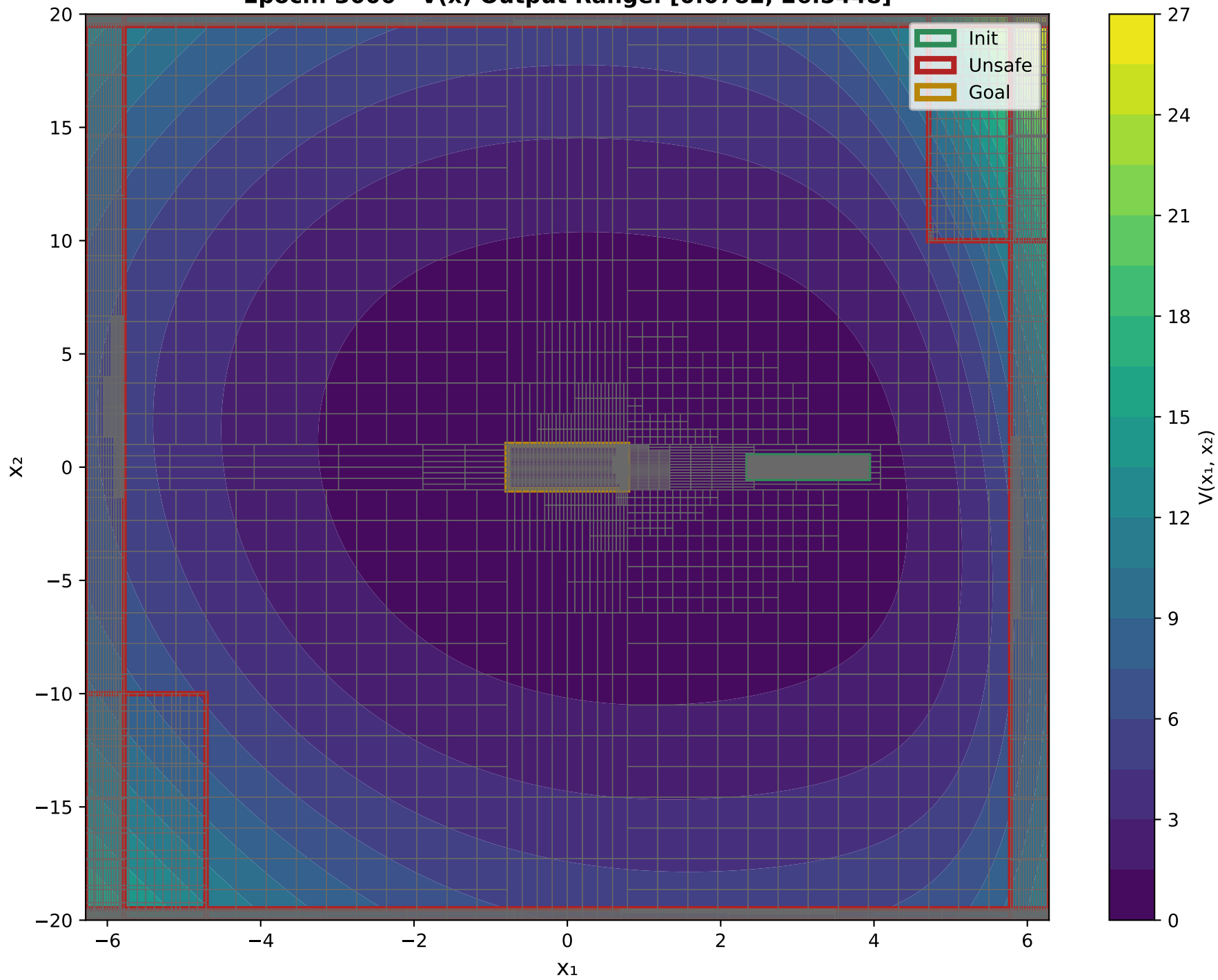
X 1 VS X 2 Epoch: 3000 - V(x) Output Range: [0.0782, 26.5448]
