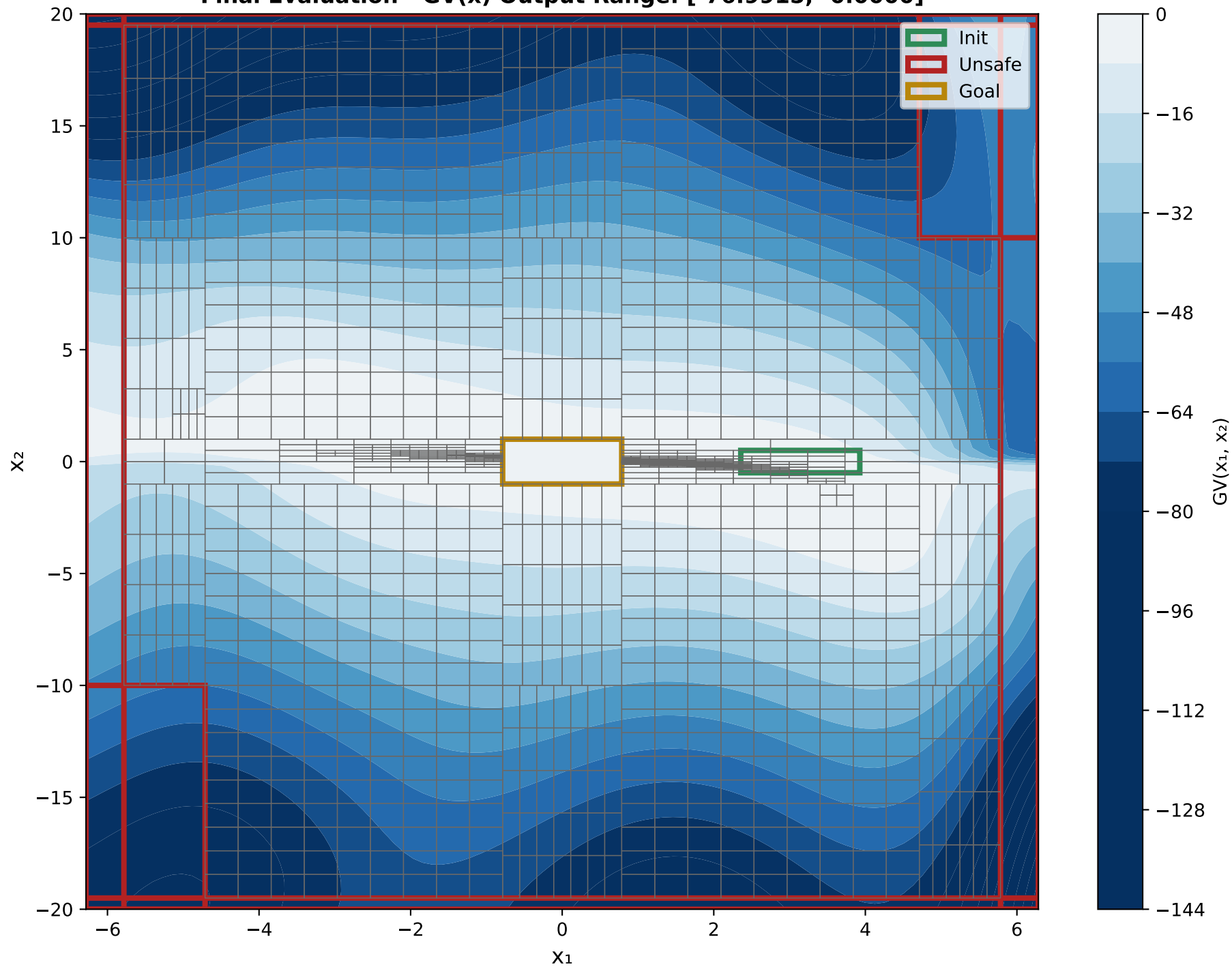
X 1 VS X 2 Final Evaluation - GV(x) Output Range: [-76.9915, -0.0000]
