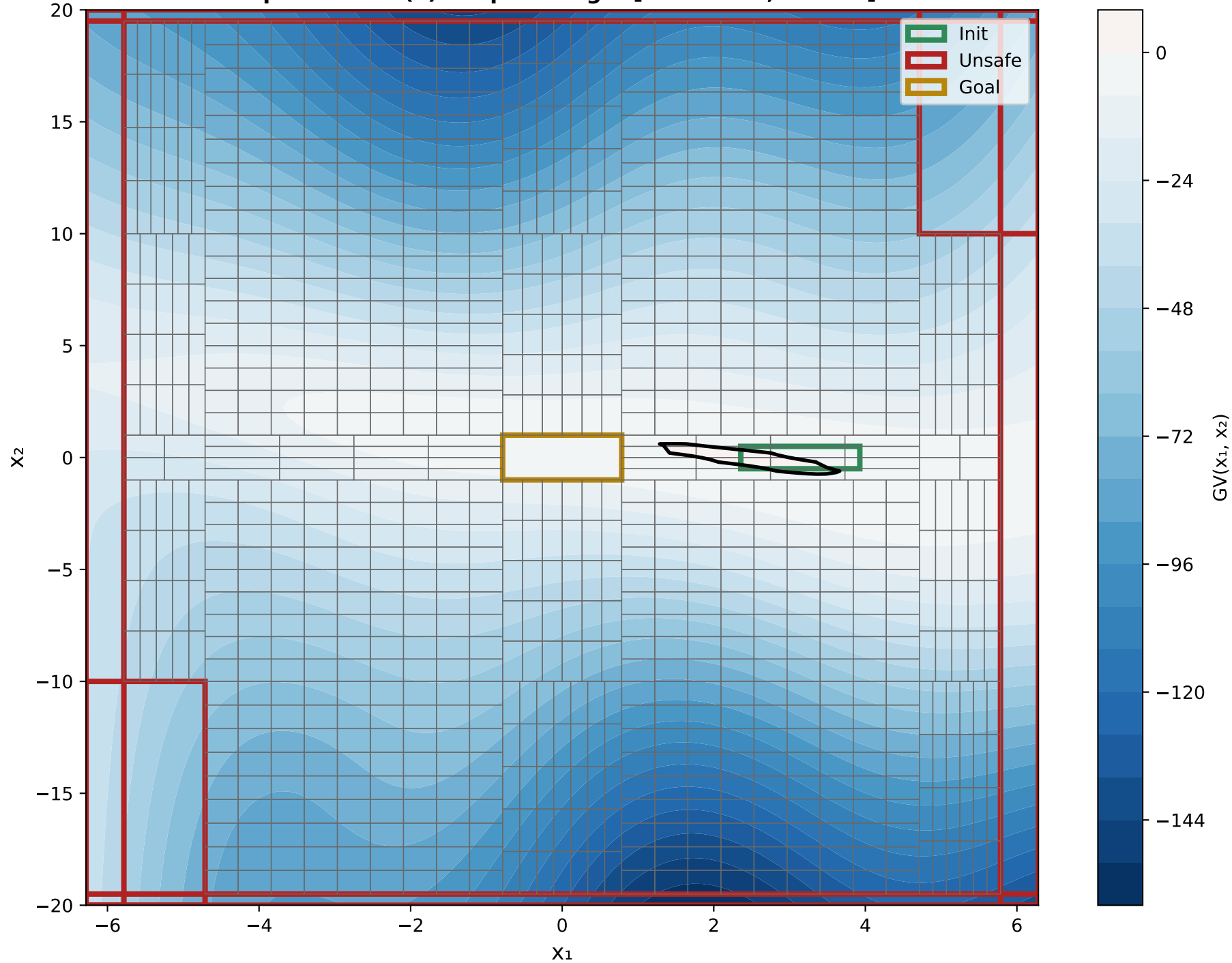
X 1 VS X 2 Epoch 0 - GV(x) Output Range: [-158.3968, 0.3096]
