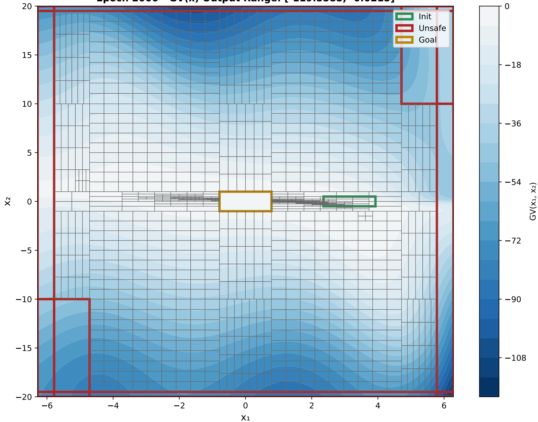
X 1 VS X 2 Epoch 2000 - GV(x) Output Range: [-119.5585, -0.0215]
