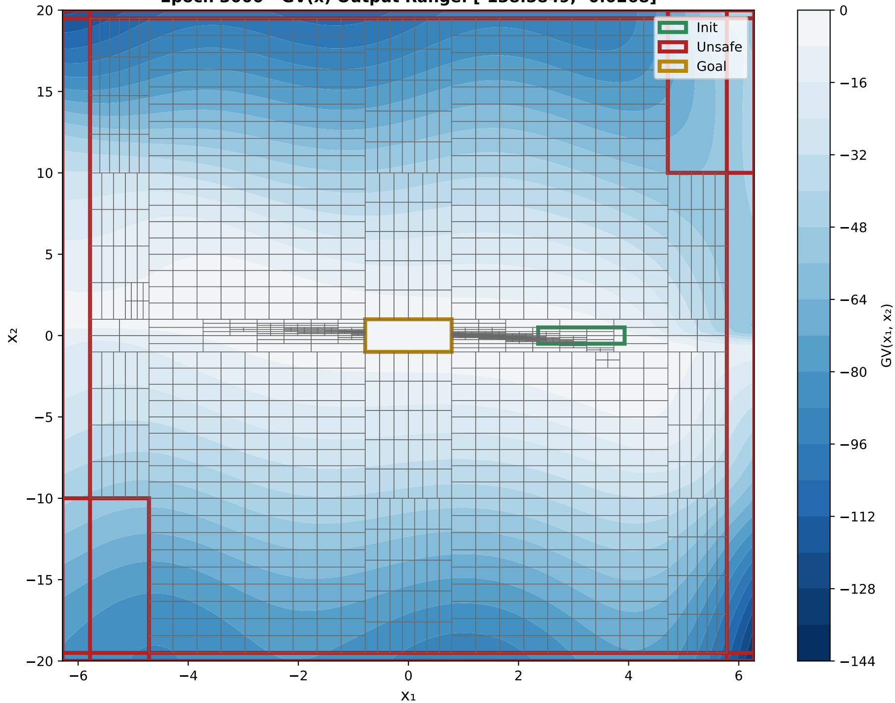
X 1 VS X 2 Epoch 3000 - GV(x) Output Range: [-138.5849, -0.0268]
