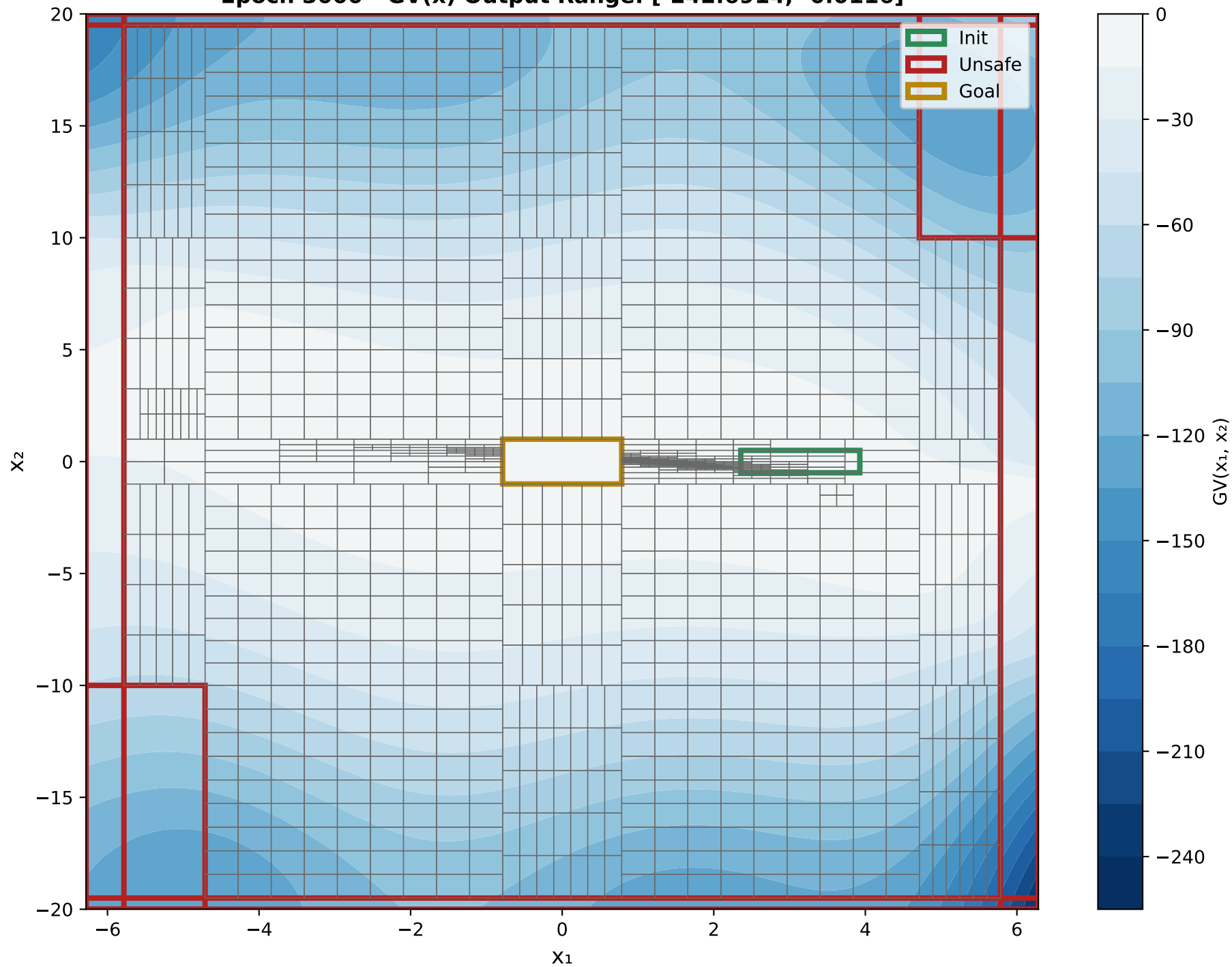
X 1 VS X 2 Epoch 3000 - GV(x) Output Range: [-242.6914, -0.0116]
