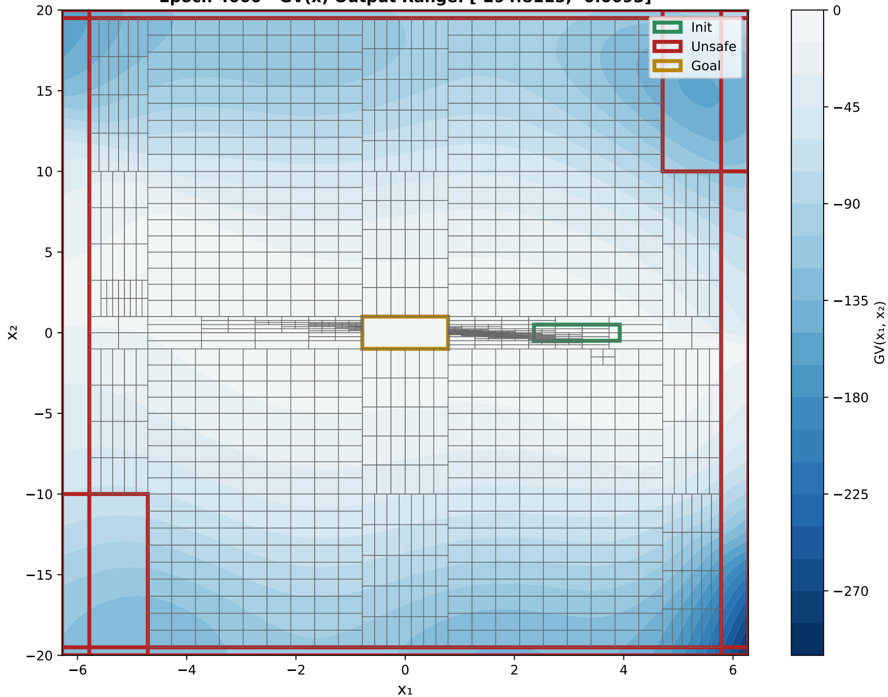
X 1 VS X 2 Epoch 4000 - GV(x) Output Range: [-294.8115, -0.0093]
