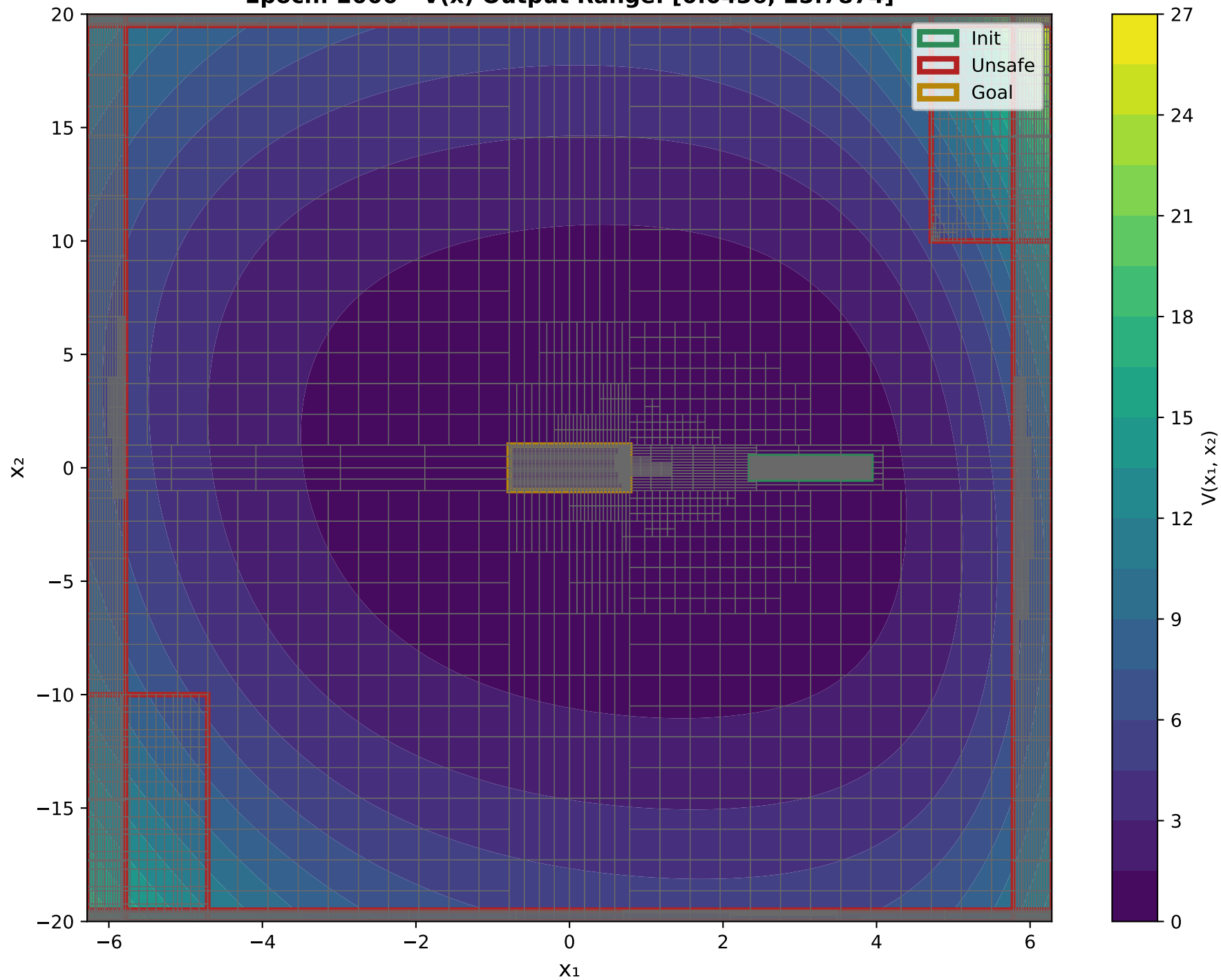
X 1 VS X 2 Epoch: 2000 - V(x) Output Range: [0.0436, 25.7874]
