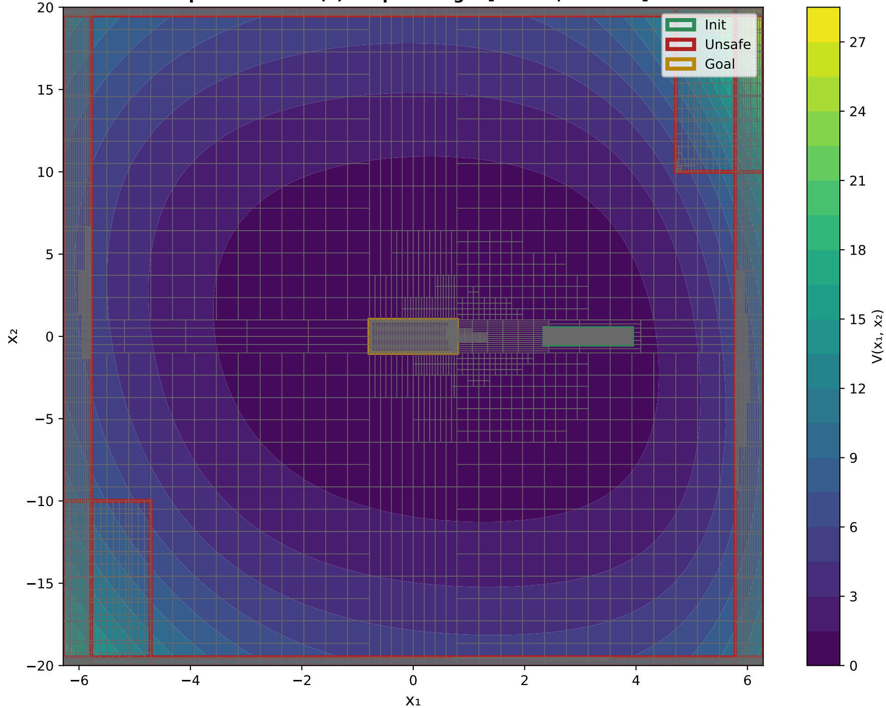
X 1 VS X 2 Epoch: 3000 - V(x) Output Range: [0.0615, 27.2362]
