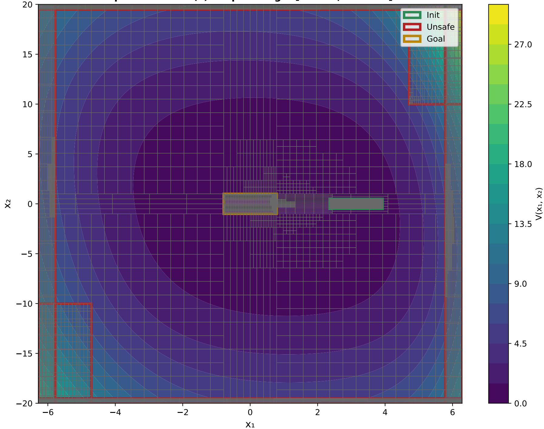
X 1 VS X 2 Epoch: 4000 - V(x) Output Range: [0.0692, 29.8056]
