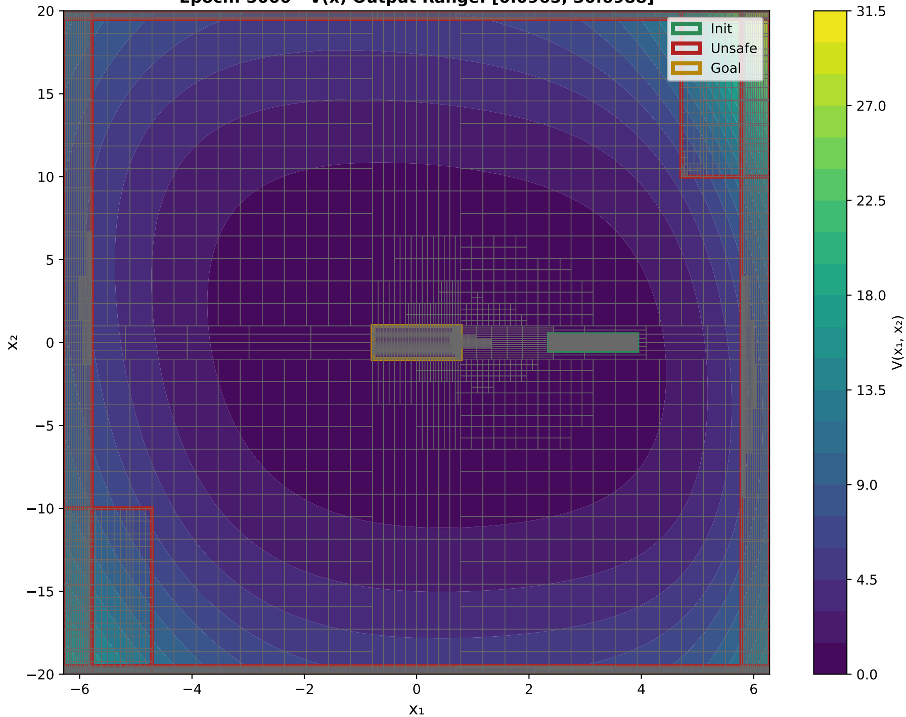
X 1 VS X 2 Epoch: 5000 - V(x) Output Range: [0.0965, 30.6988]
