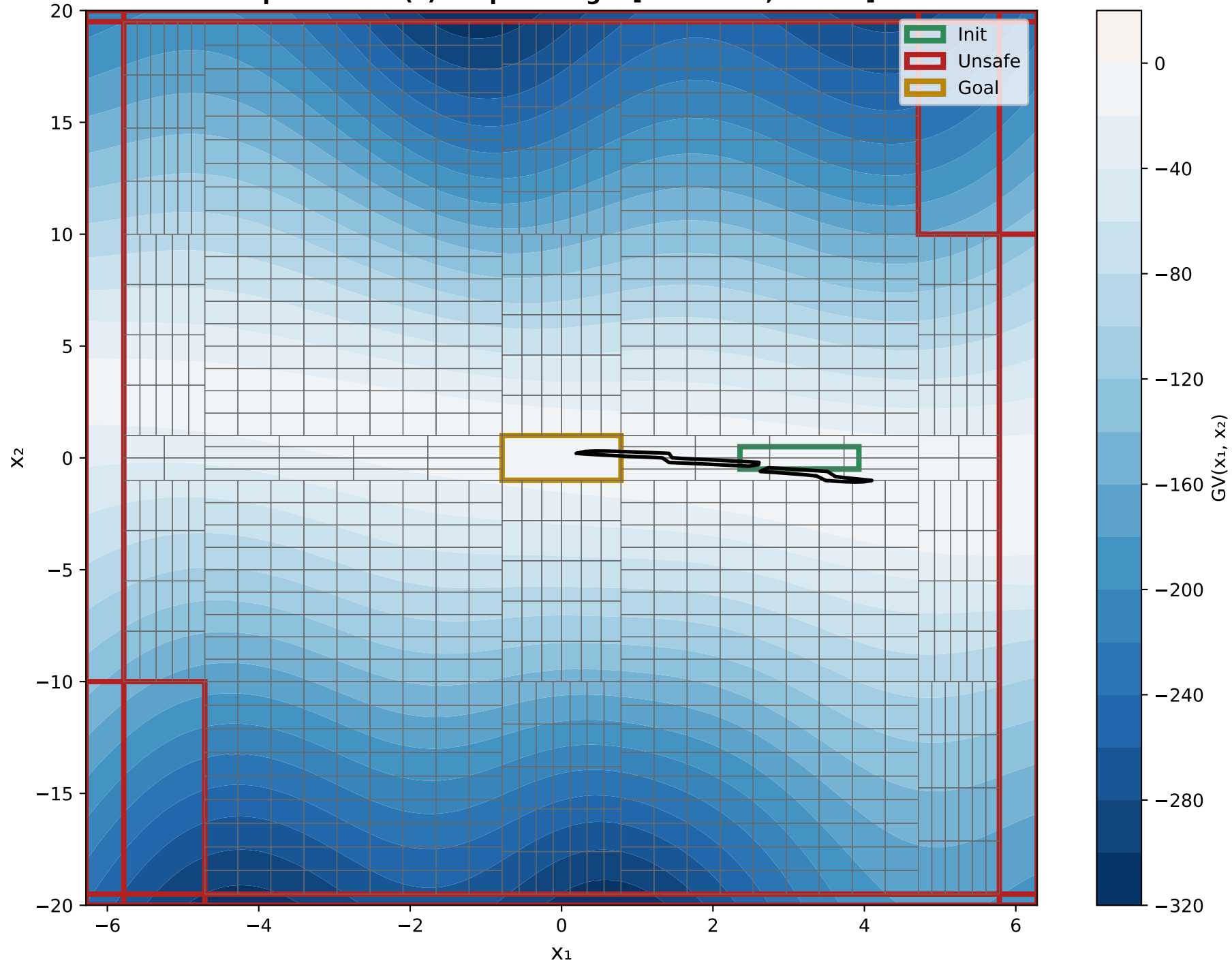
X 1 VS X 2 Epoch 0 - GV(x) Output Range: [-316.3974, 0.3045]
