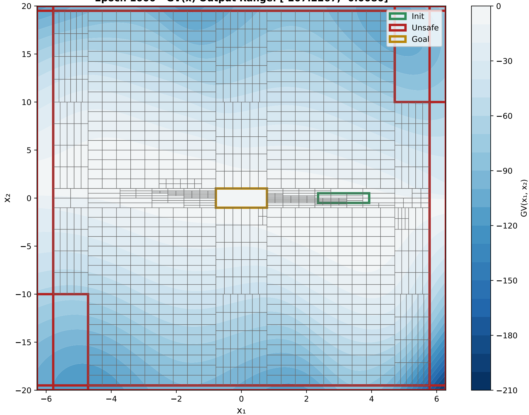
X 1 VS X 2 Epoch 1000 - GV(x) Output Range: [-207.2267, -0.0080]
