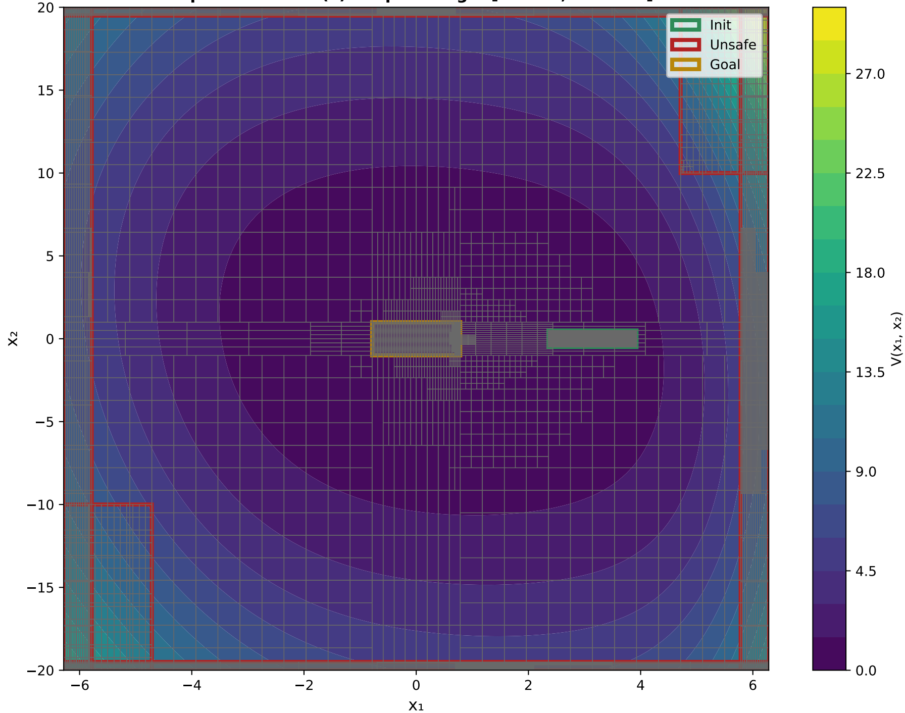
X 1 VS X 2 Epoch: 3000 - V(x) Output Range: [0.0874, 29.5603]
