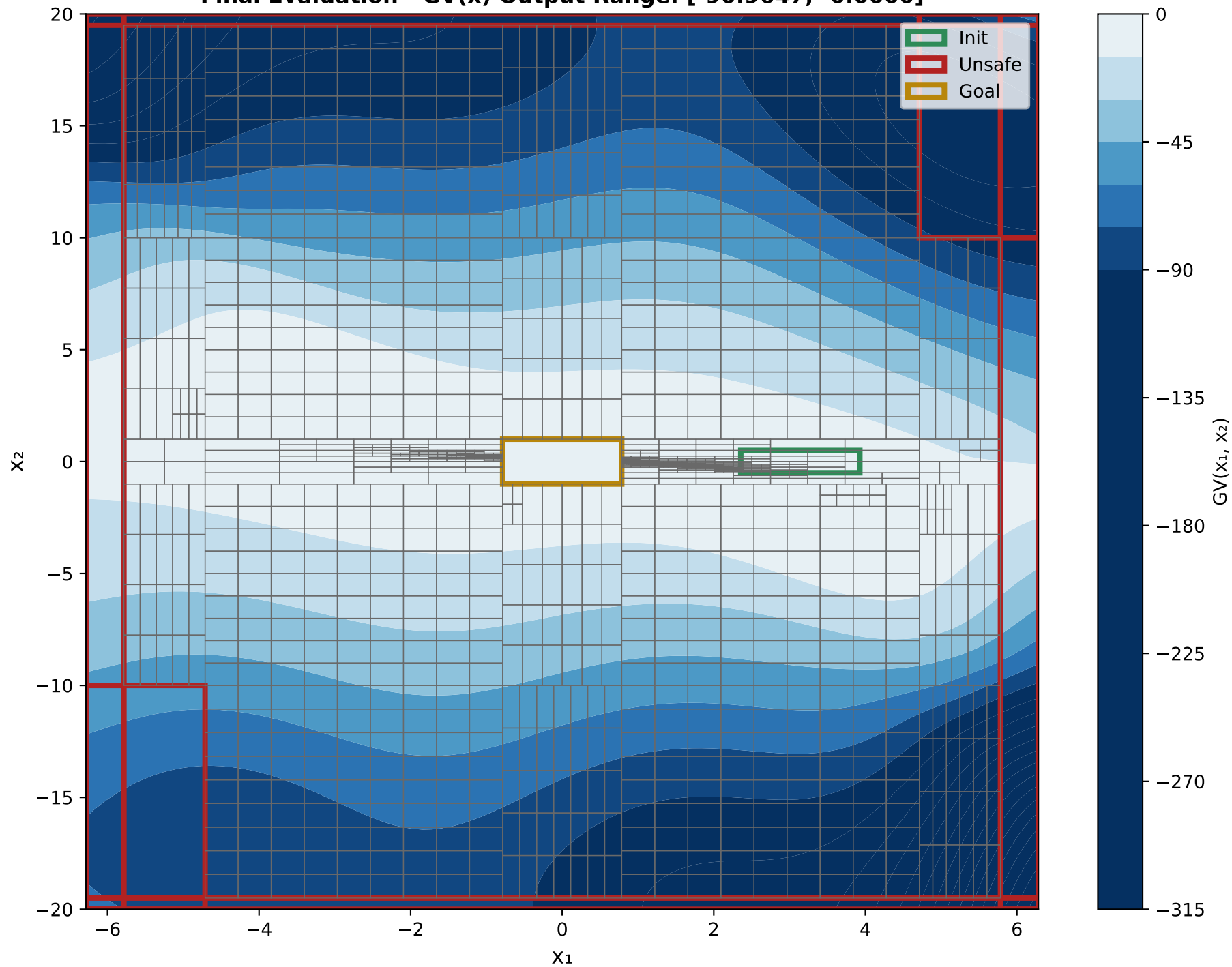
X 1 VS X 2 Final Evaluation - GV(x) Output Range: [-90.9647, -0.0000]
