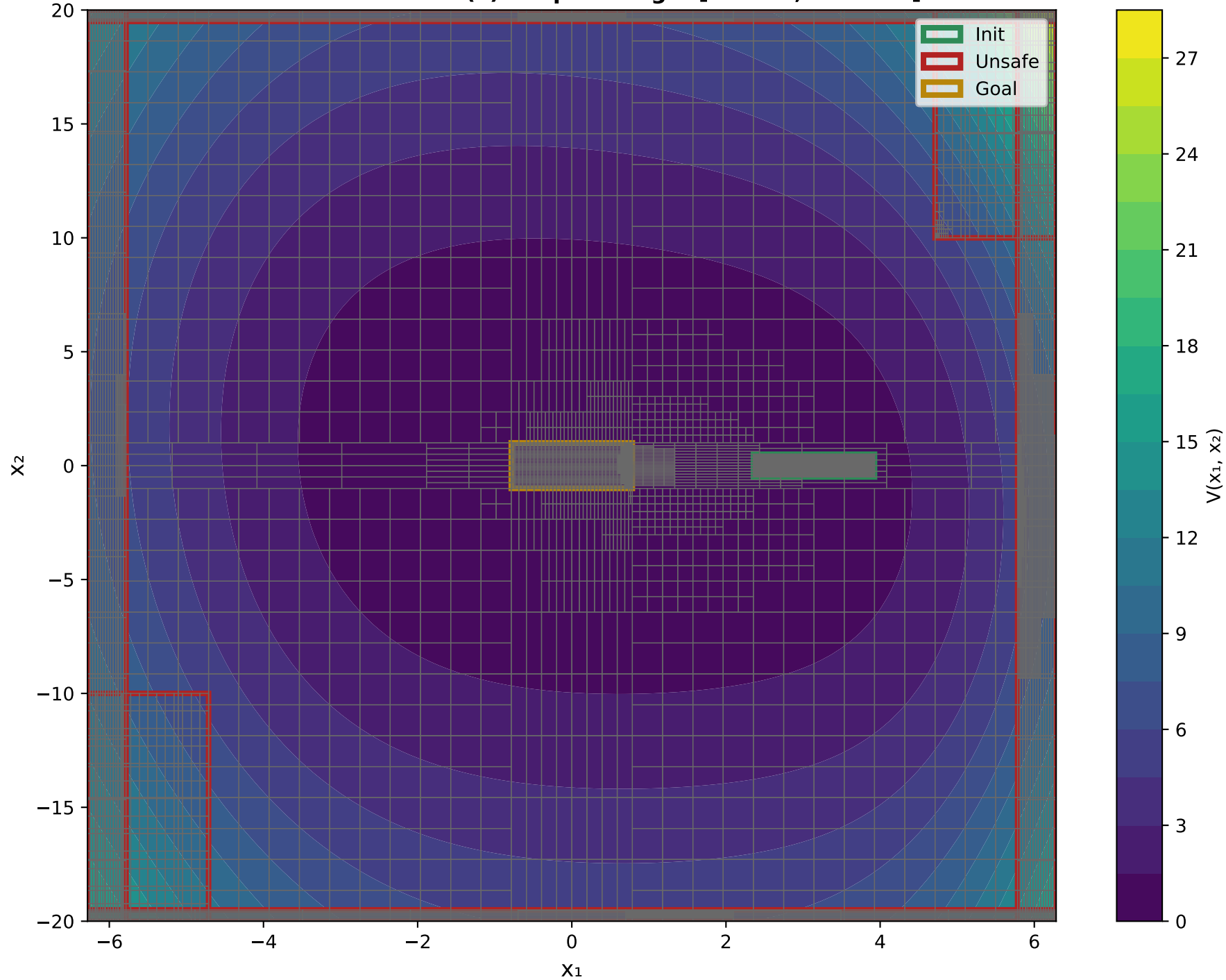
X 1 VS X 2 Final Evaluation - V(x) Output Range: [0.0979, 27.2847]
