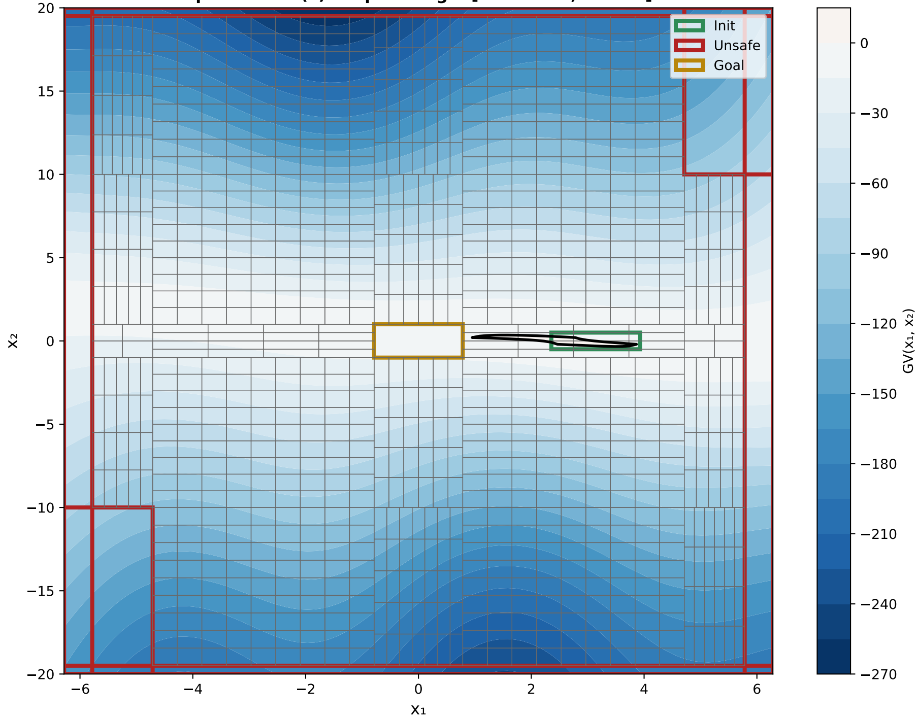
X 1 VS X 2 Epoch 0 - GV(x) Output Range: [-268.1605, 0.2846]
