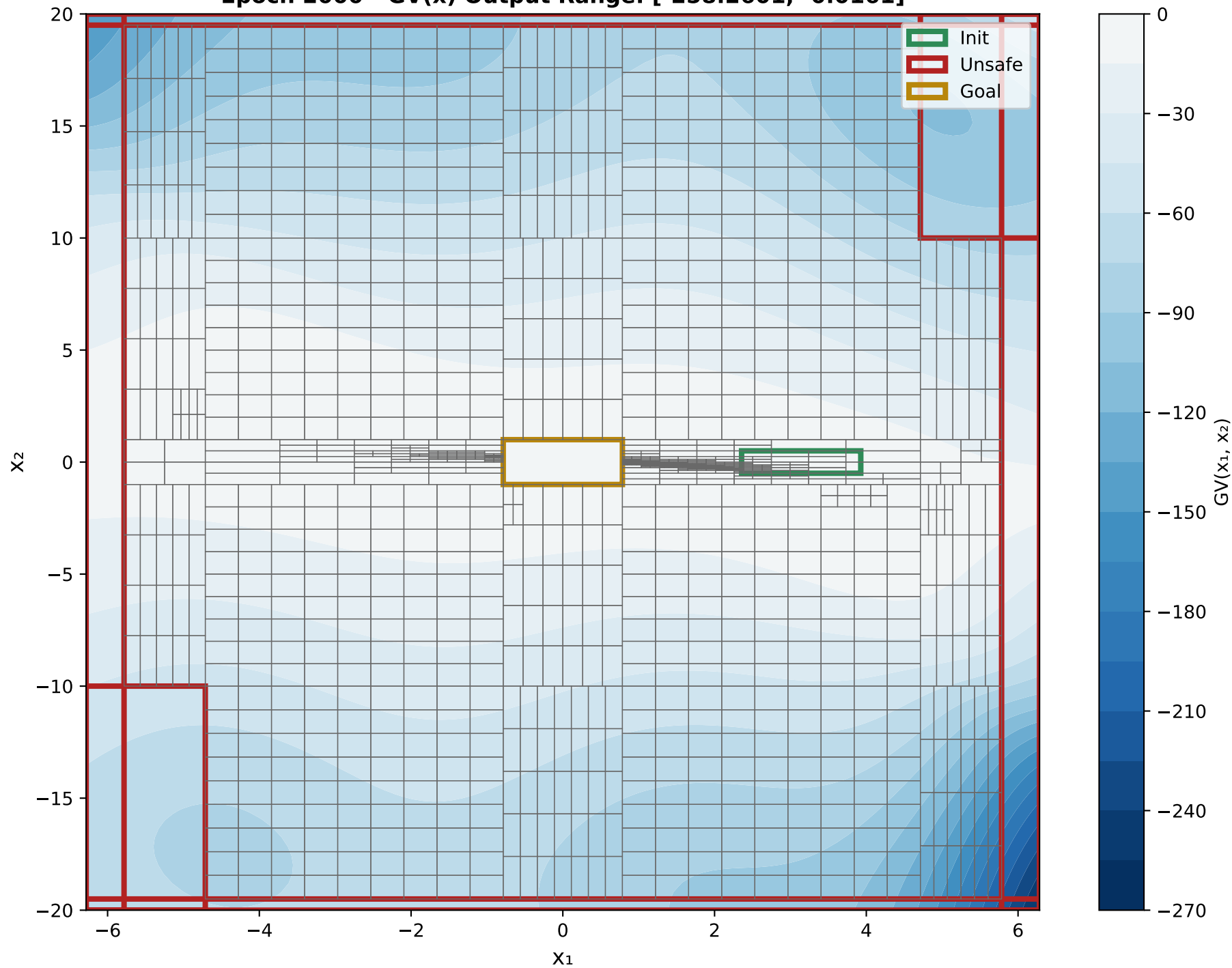
X 1 VS X 2 Epoch 2000 - GV(x) Output Range: [-258.2601, -0.0161]
