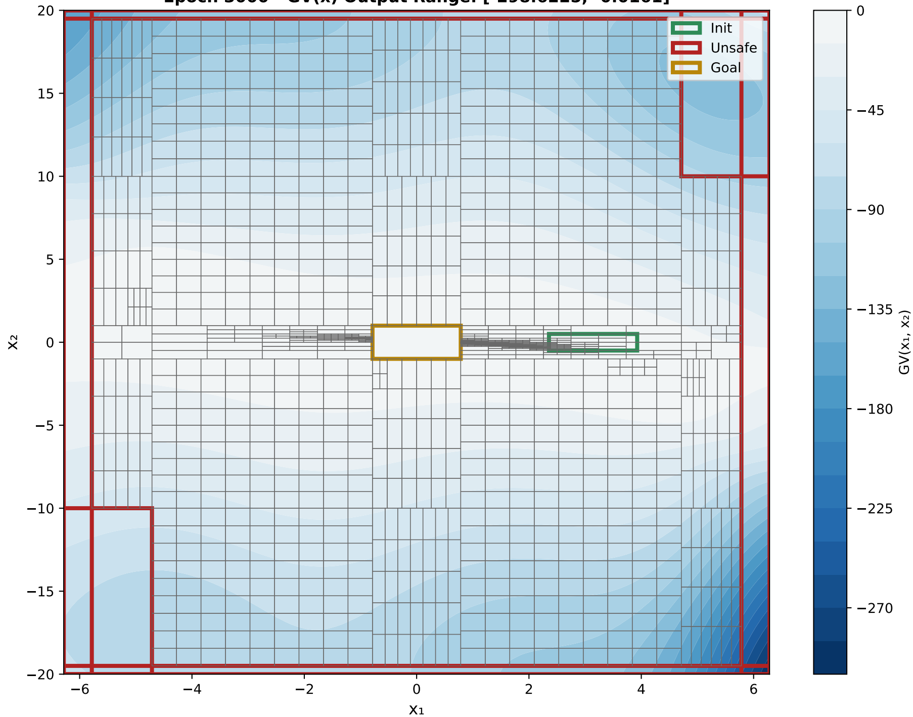
X 1 VS X 2 Epoch 3000 - GV(x) Output Range: [-298.6225, -0.0161]
