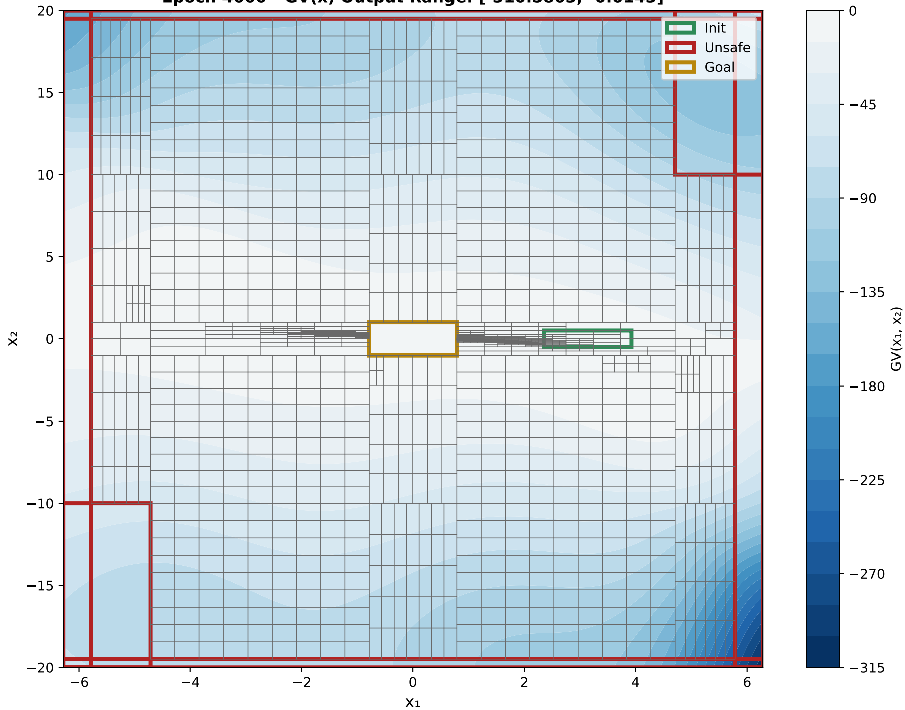
X 1 VS X 2 Epoch 4000 - GV(x) Output Range: [-310.5803, -0.0143]
