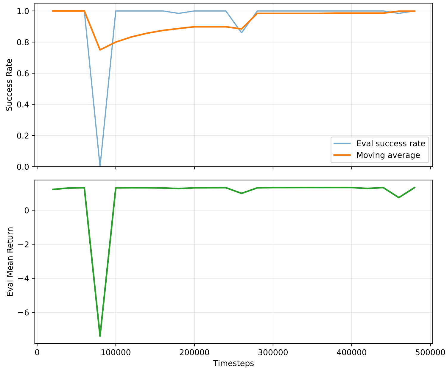
SB3 DDPG Training History (Off-the-shelf)
