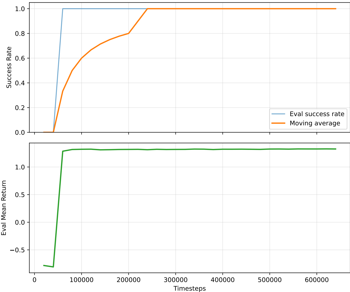
SB3 PPO Training History (Off-the-shelf)
