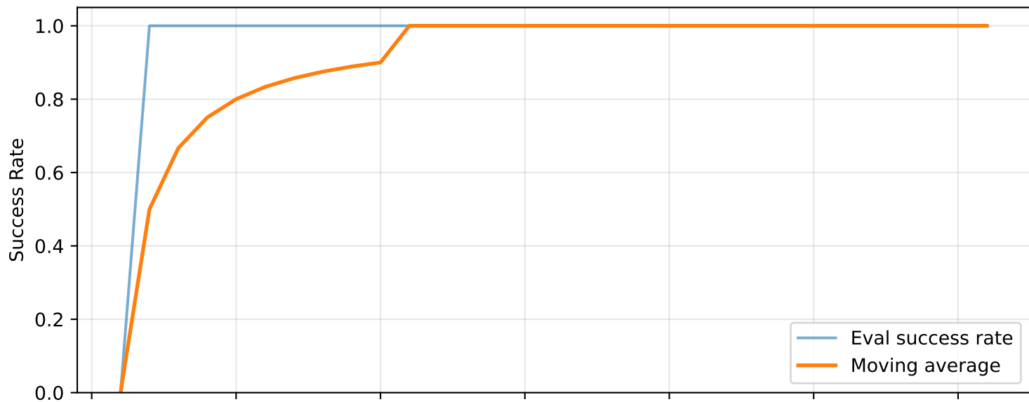
SB3 PPO (Energy-Regularized) Training History
