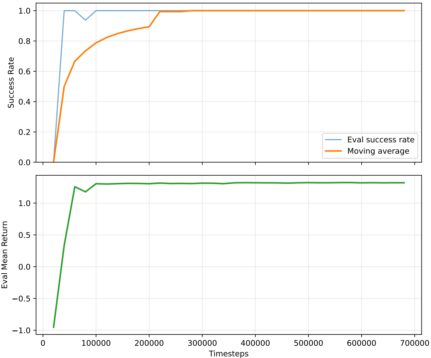
SB3 PPO+RPO Training History (Off-the-shelf)
