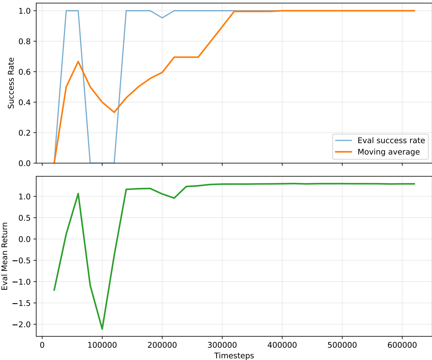
SB3 SAC Training History (Off-the-shelf)
