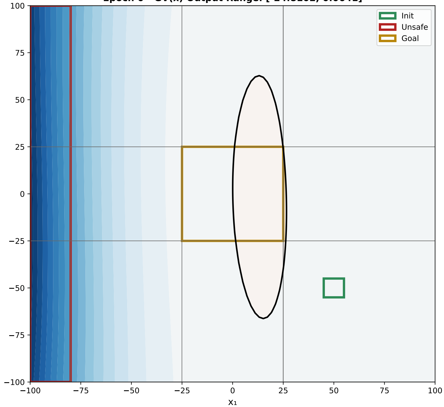
X 1 VS X 2 Epoch 0 - GV(x) Output Range: [-24.8102, 0.0641]
