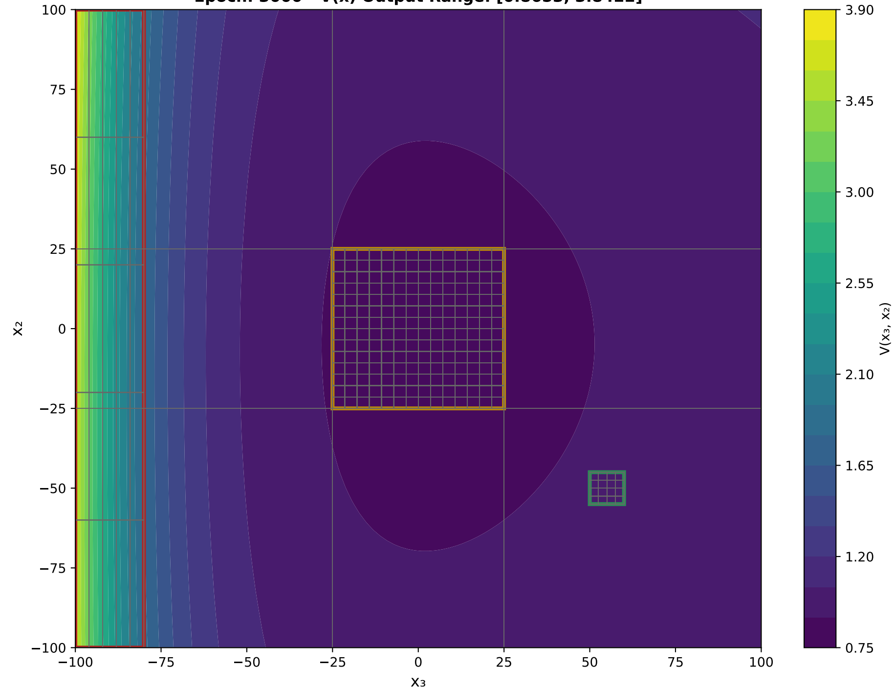
X 3 VS X 2 Epoch: 3000 - V(x) Output Range: [0.8653, 3.8422]
