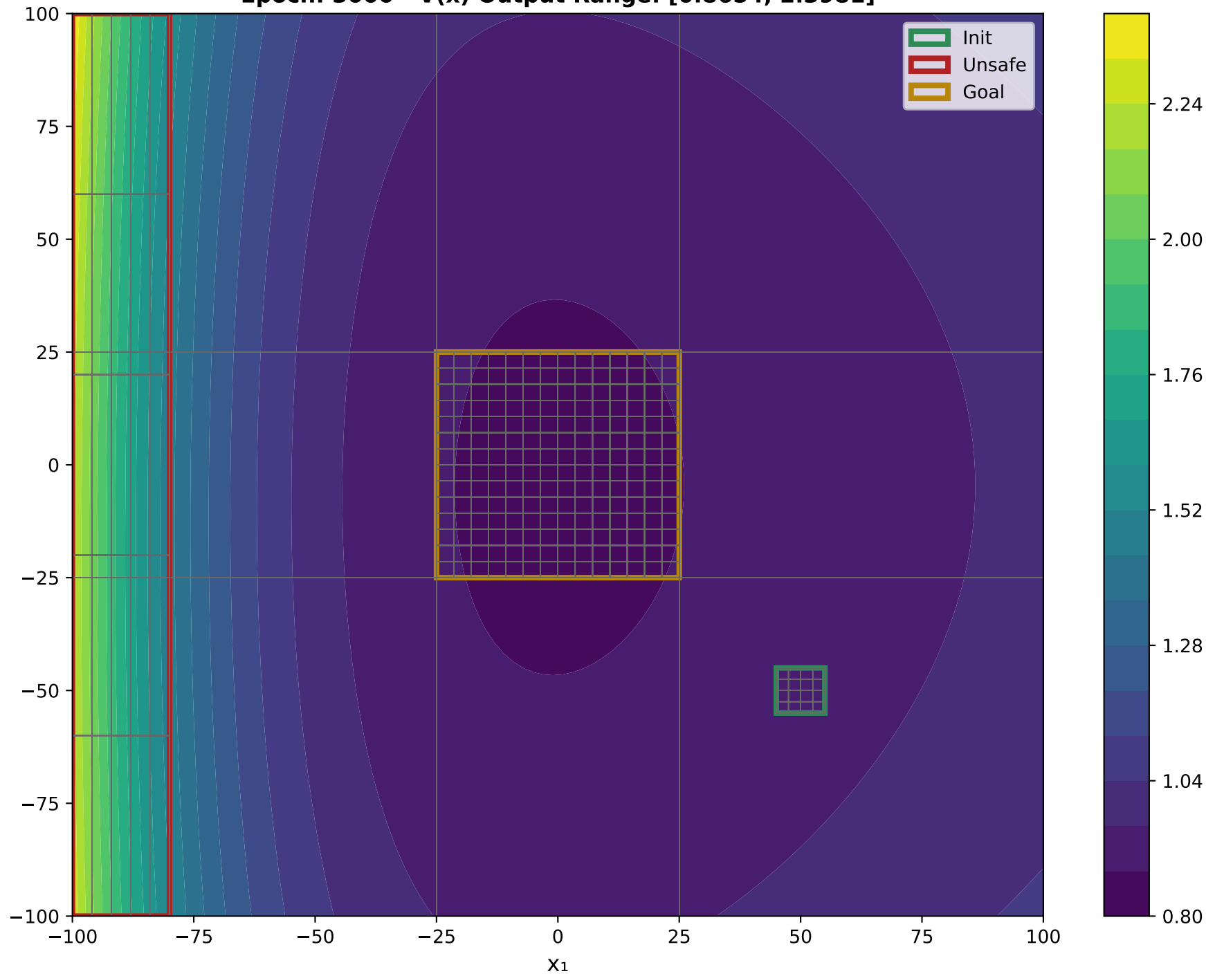
X 1 VS X 2 Epoch: 3000 - V(x) Output Range: [0.8654, 2.3981]
