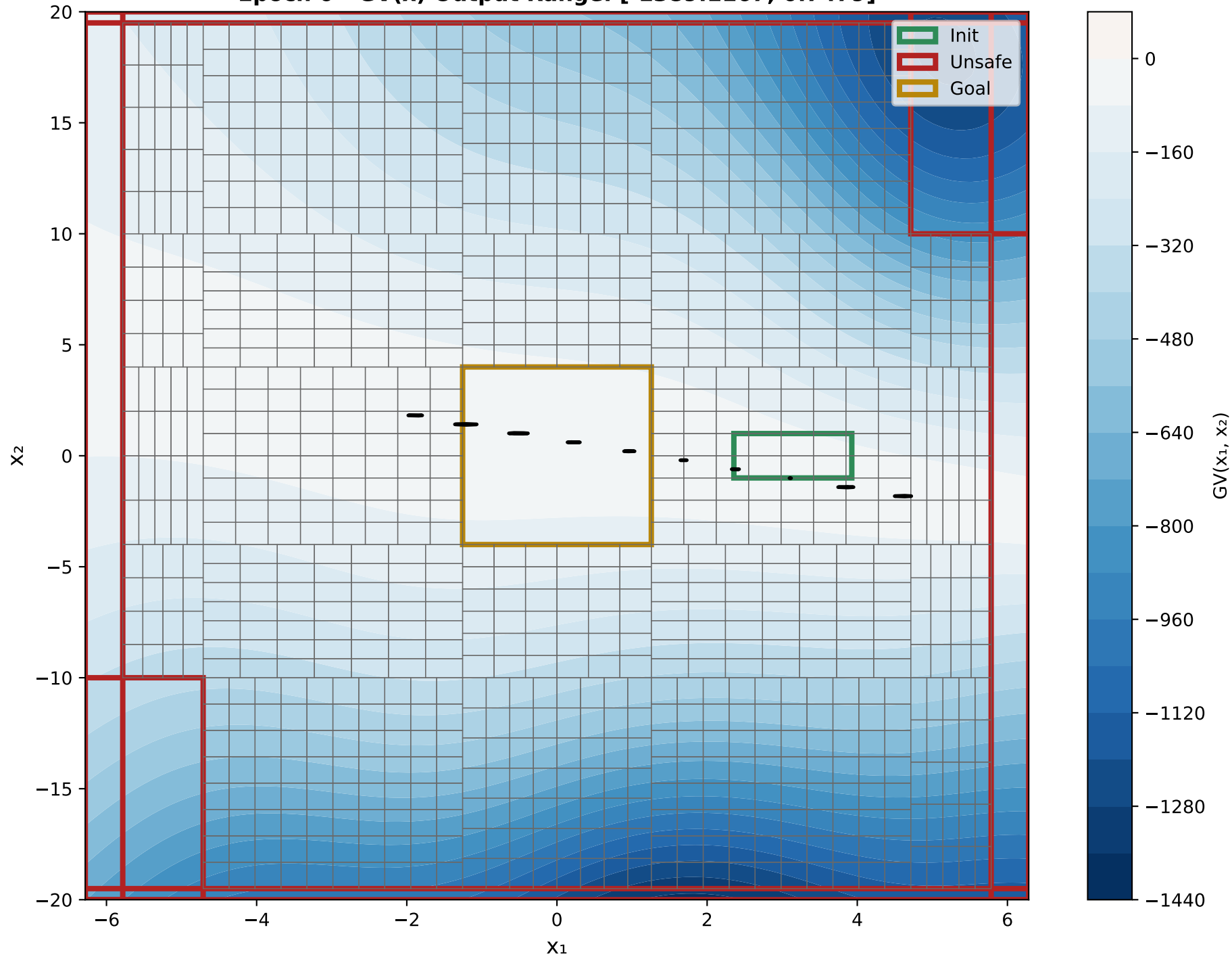
X 1 VS X 2 Epoch 0 - GV(x) Output Range: [-1389.1167, 0.7479]
