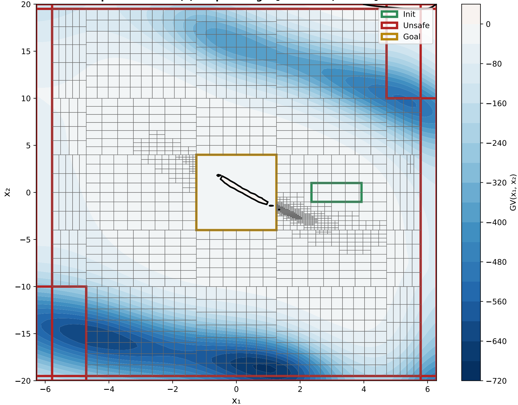
X 1 VS X 2 Epoch 2000 - GV(x) Output Range: [-688.6480, 9.4598]
