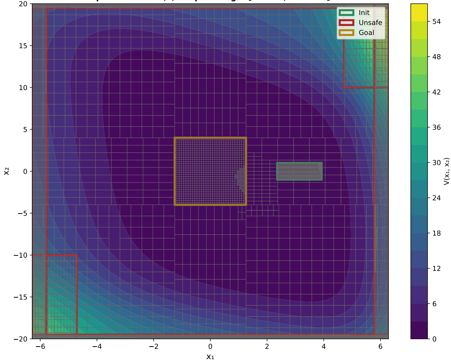
X 1 VS X 2 Epoch: 1000 - V(x) Output Range: [0.0261, 54.9864]
