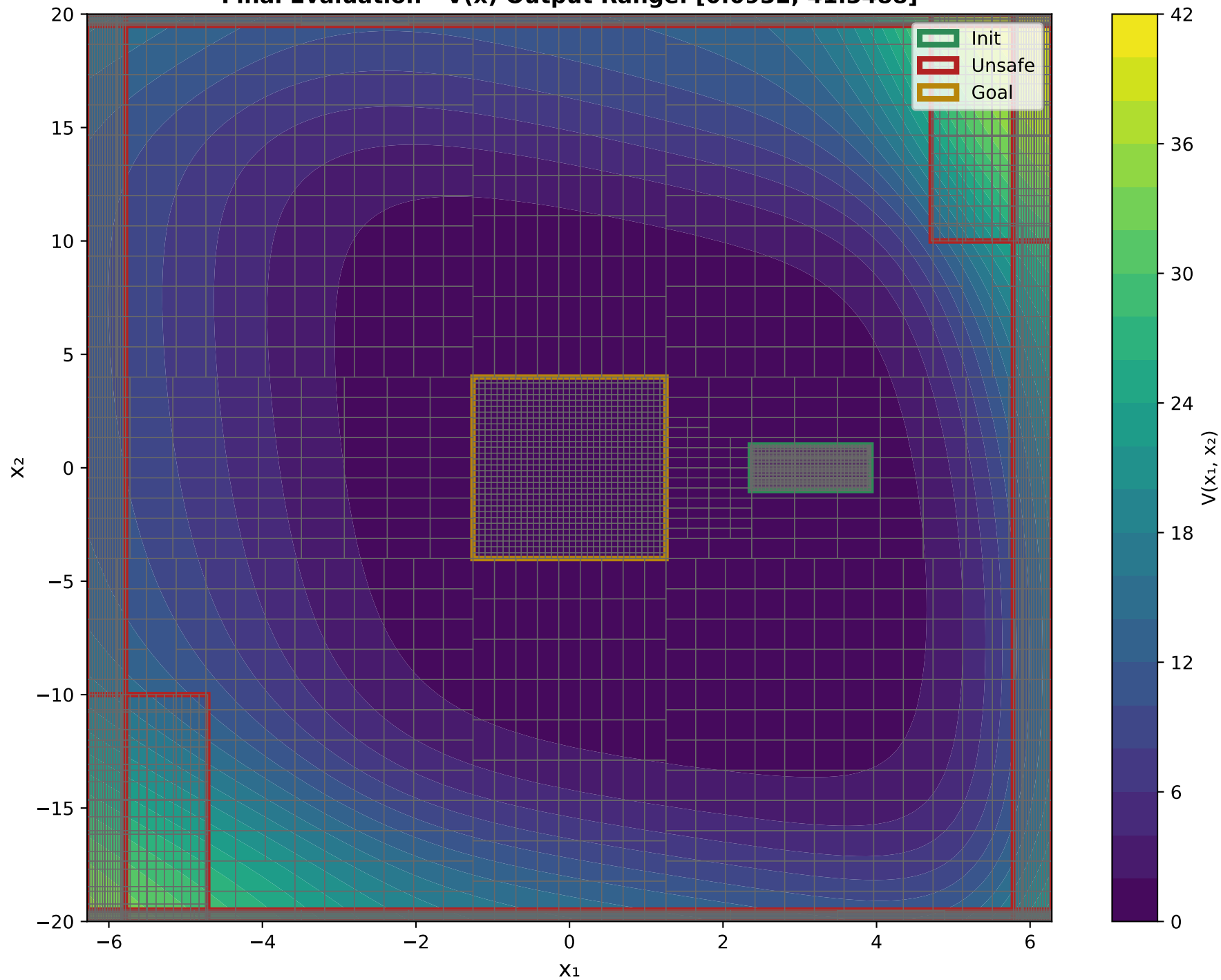
X 1 VS X 2 Final Evaluation - V(x) Output Range: [0.0932, 41.3488]
