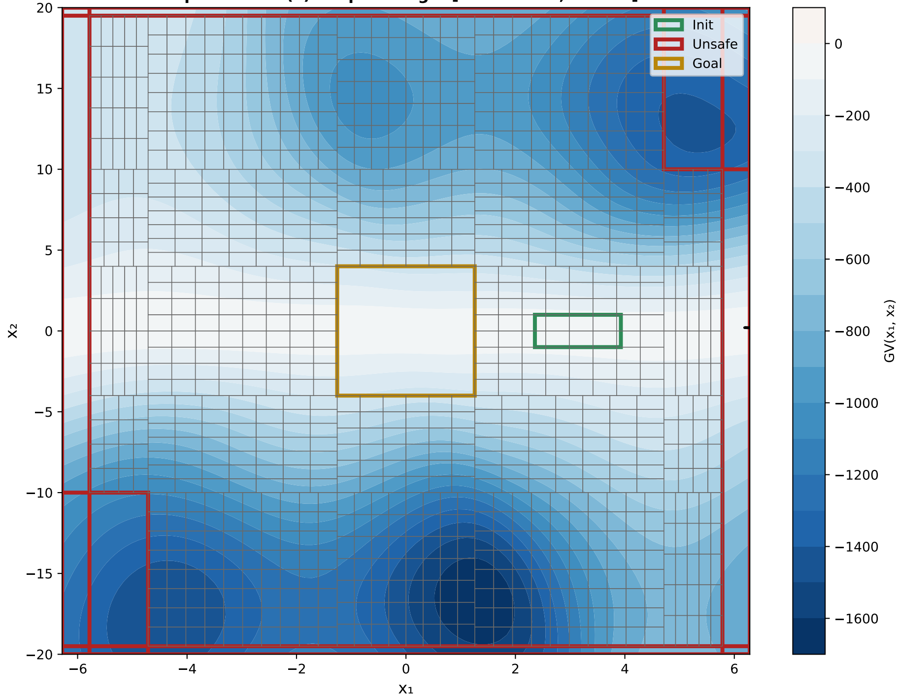
X 1 VS X 2 Epoch 0 - GV(x) Output Range: [-1683.3583, 0.3725]
