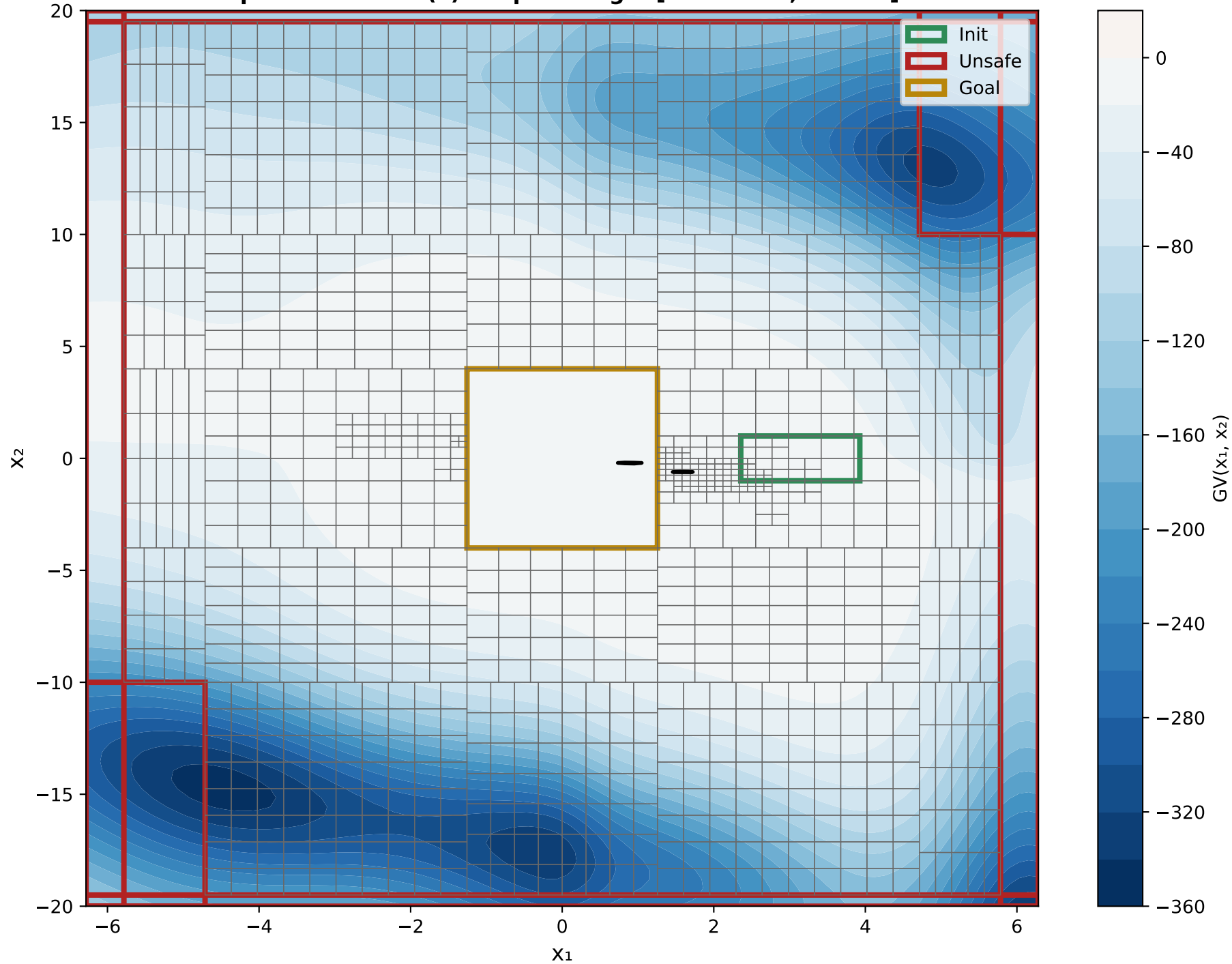
X 1 VS X 2 Epoch 1000 - GV(x) Output Range: [-349.9884, 0.0074]
