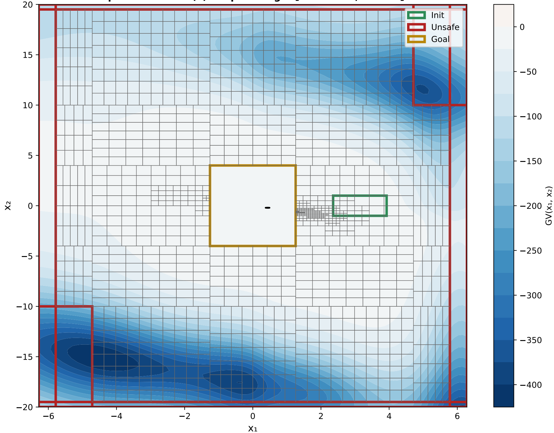
X 1 VS X 2 Epoch 2000 - GV(x) Output Range: [-423.3028, 0.0037]
