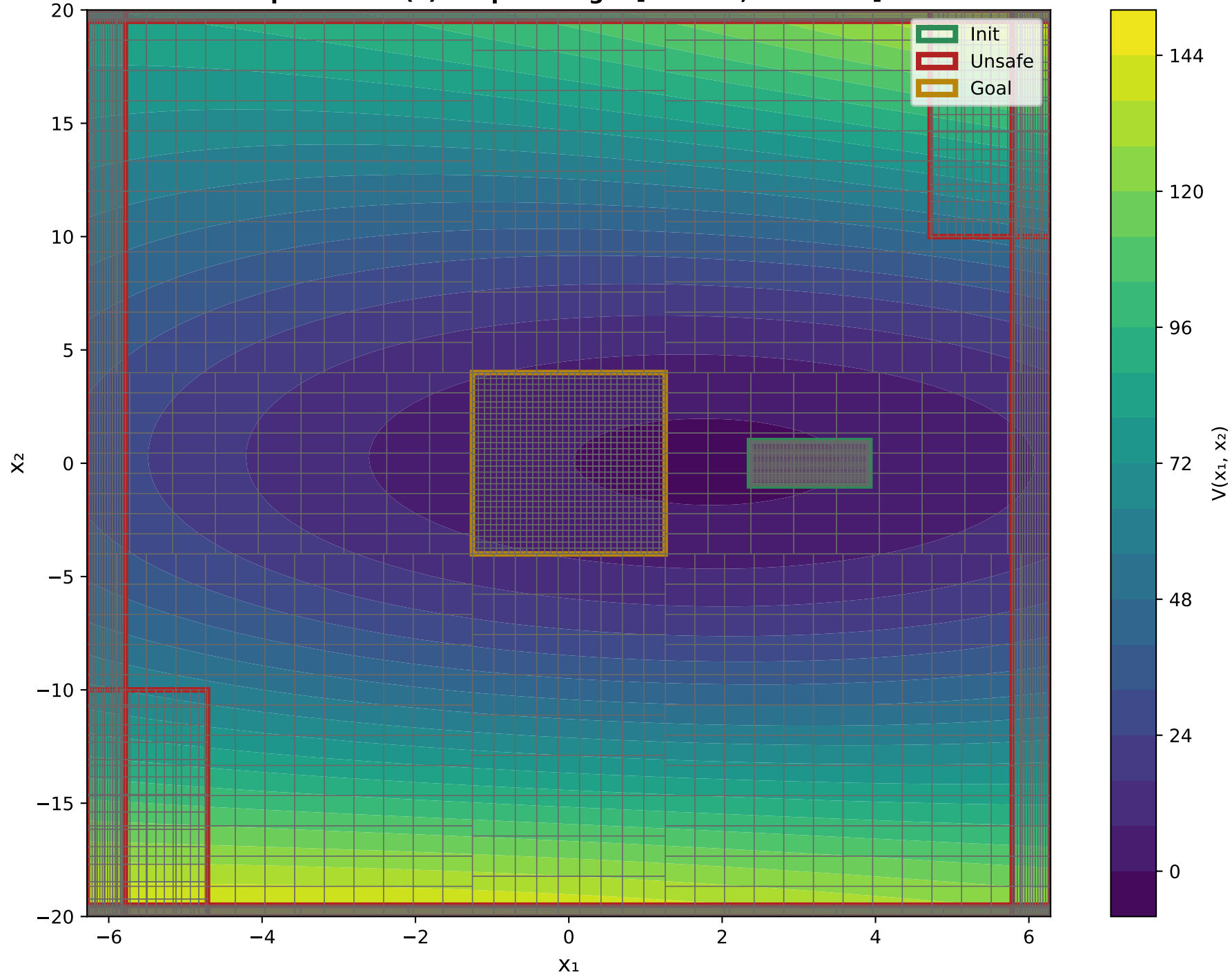
X 1 VS X 2 Epoch: 0 - V(x) Output Range: [-1.5504, 148.9415]
