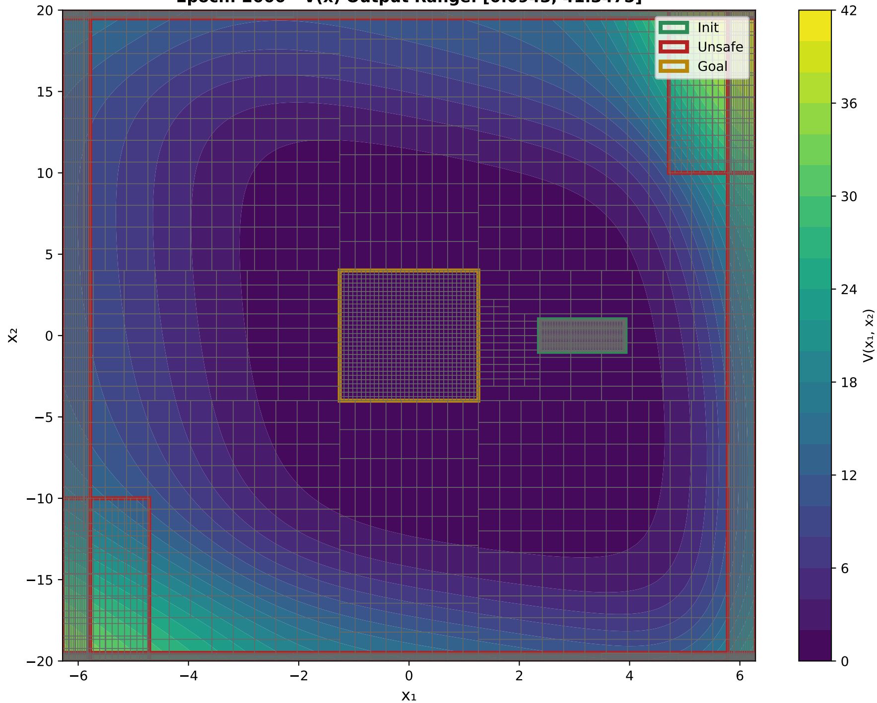
X 1 VS X 2 Epoch: 2000 - V(x) Output Range: [0.0943, 41.3475]
