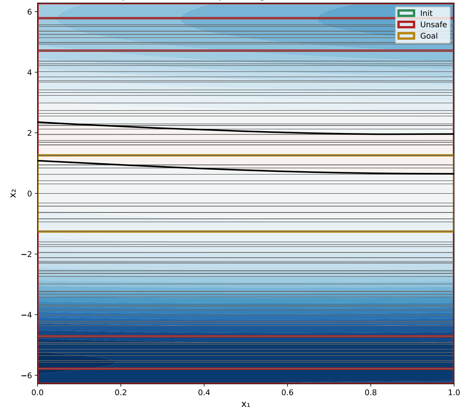
X 1 VS X 2 Epoch 0 - GV(x) Output Range: [-91.1643, 1.3779]
