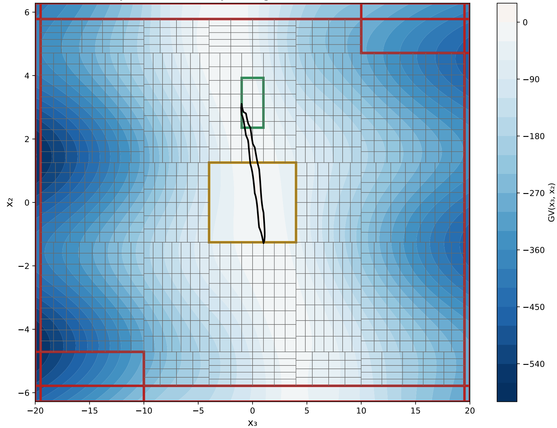
X 3 VS X 2 Epoch 0 - GV(x) Output Range: [-572.7979, 1.1954]
