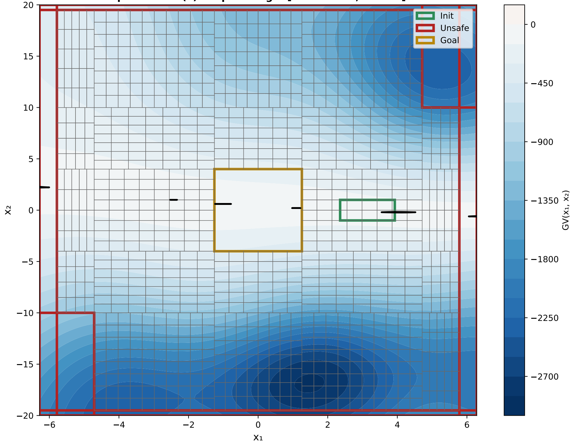
X 1 VS X 2 Epoch 0 - GV(x) Output Range: [-2879.3486, 3.2752]
