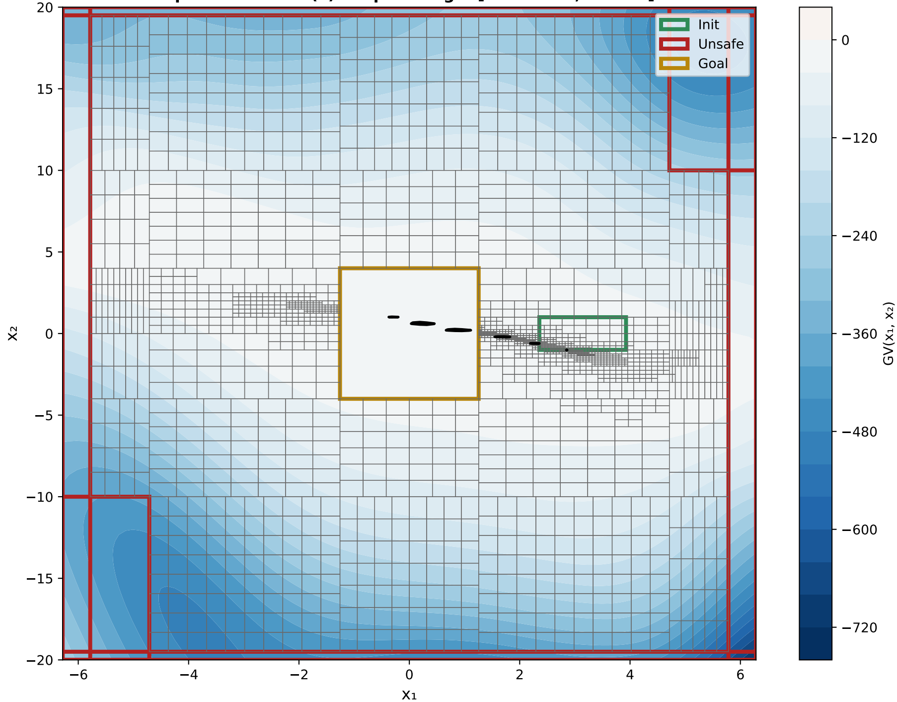
X 1 VS X 2 Epoch 2000 - GV(x) Output Range: [-729.3860, 0.2369]
