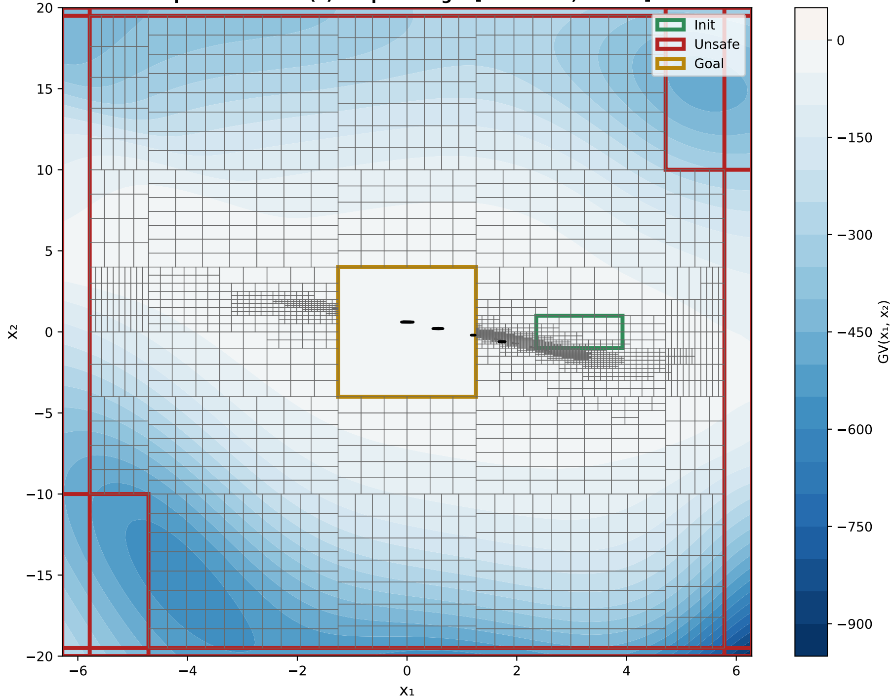
X 1 VS X 2 Epoch 3000 - GV(x) Output Range: [-941.1375, 0.0564]
