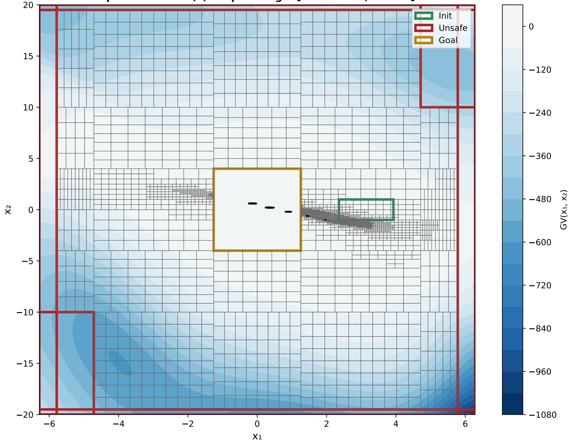
X 1 VS X 2 Epoch 4000 - GV(x) Output Range: [-1072.7000, 0.0809]
